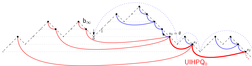
Figure 9: The construction of the UIHPQ_0 from a uniform infinite bridge b_\infty . The spine is shown in bold red arcs. The trees on the left of the spine are drawn in blue and enclosed by dotted blue half-circles, which indicate the corresponding excursions of b_\infty encoding these trees. The trees on the right of the spine are drawn in red, as the spine itself.
