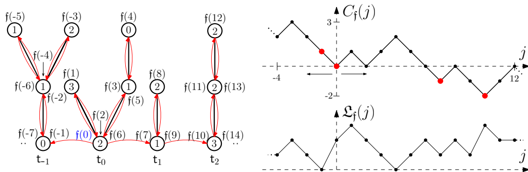
Figure 6: Contour and label functions C_f and \mathcal{L}_f of an element ((f, l), b) \in \mathfrak{F}_\infty \times \mathfrak{B}_\infty . The left side depicts the two-sided contour exploration of f . The labels are given by \mathcal{L}_f(j) , where now j \in \mathbb{Z} . The values of the infinite bridge b at its first three down-steps to the right of 0 read here b(d^\downarrow(1)) = 2 , b(d^\downarrow(2)) = 1 and b(d^\downarrow(3)) = 3 , while the first down-step to the left of zero has value b(d^\downarrow(-1)) = 0 . The arrows below the contour function indicate the direction of the encoding, and the red dots mark again the encoding of a new tree.
