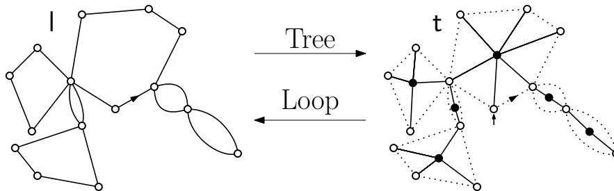
Figure 4: A looptree and the associated tree of components.
