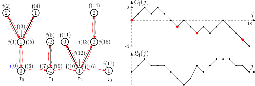
Figure 5: Contour and label functions C_f and \mathcal{L}_f of an element ((f, l), b) \in \mathfrak{F}_4^7 \times \mathfrak{B}_4 . The left side depicts the contour exploration of f . The labels on the vertices are given by \mathcal{L}_f(j) , j = 0, \dots, 18 . Note that the values of b at its four down-steps are equal to the values of \mathcal{L}_f at the tree roots: In this example, we have b(d^\downarrow(1)) = 0 , b(d^\downarrow(2)) = -1 , and b(d^\downarrow(3)) = b(d^\downarrow(4)) = 1 . The red dots on the right indicate the encoding of a new tree.
