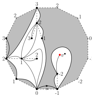
Figure 7: A representation of an element ((f, l), b) \in \mathfrak{F}_6^6 \times \mathfrak{B}_6 in the plane and the associated rooted pointed quadrangulation (q, v^\bullet) = \Phi_n((f, l), b) . The distinguished vertex of the cycle is the down-most vertex labeled 0. The trees are grafted to the 6 down-steps of b (here, d^\downarrow(1) = 0 , d^\downarrow(2) = 1 , d^\downarrow(3) = 7 , d^\downarrow(4) = 9 , d^\downarrow(5) = 10 , and d^\downarrow(6) = 11 ). The tree edges are indicated by the dashed lines in the interior of the cycle. Note that three trees (those above the first, fourth and sixth down-step) consist of a single vertex. The labels in a tree are shifted by the bridge value of the down-step above which the tree is attached. Note that the 12 boundary edges of the cycle are in a order-preserving correspondence with the 12 boundary edges of q . (The two edges of q which lie entirely in the outer face are counted twice.)
