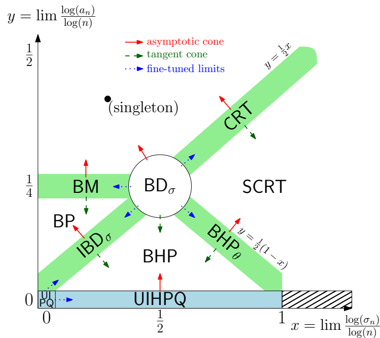
Figure 1: In [8], all possible limits for the rescaled spaces (V(Q_n^{\sigma_n}), a_n^{-1}d_{gr}, \rho_n) are discussed. The x -axis represents the limit values for the logarithm of the boundary length \log(\sigma_n)/\log(n) in units of \log(n) , and the y -axis corresponds to the limit of the logarithm of the scaling factor \log(a_n)/\log(n) in units of \log(n) . The focus of this paper lies on the hashed region.
