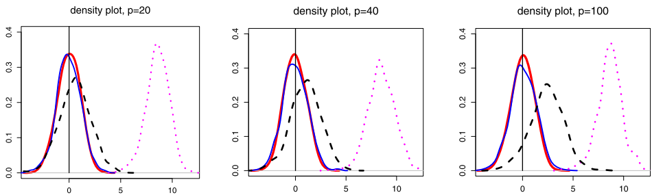
FIG. 2. The kernel density plots of the statistic, v_n \equiv \sigma_n^{-1} \sqrt{n}(\hat{\tau} - \tau^0) , for Model 1, where the estimated average treatments effects are calculated using the oracle estimate (red thick curves), the sparse_dim estimate (blue thin curves), the full_dim estimate (black dashed curves) and the sparse_linear estimate (magenta dotted curves).
