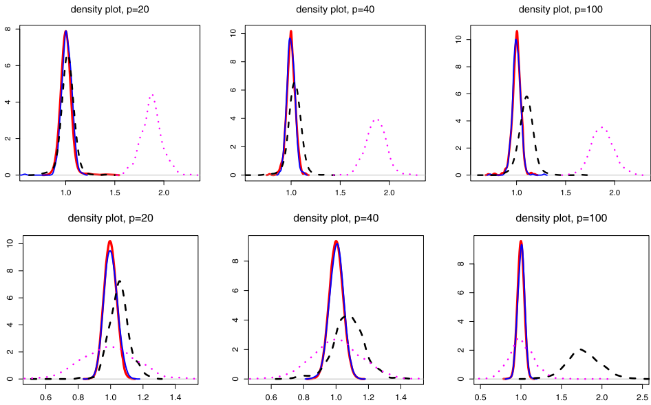
FIG. 1. The kernel density plots of the estimated average treatments effects, \hat{\tau} , calculated using the oracle estimate (red thick curves), the sparse_dim estimate (blue thin curves), the full_dim estimate (black dashed curves) and the sparse_linear estimate (magenta dotted curves); the upper and lower panels correspond to Model 1 and Model 2.
