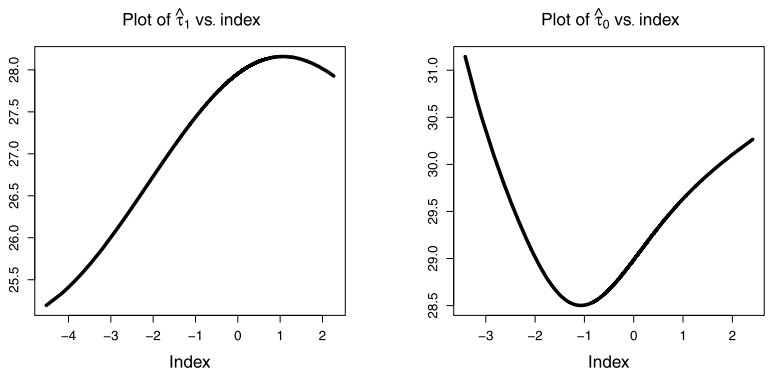
FIG. 3. The plots of \hat{\tau}_1 for the smoking group and \hat{\tau}_0 for the nonsmoking group, respectively, versus the estimated index value \hat{\mathbf{V}}^T X_i .
