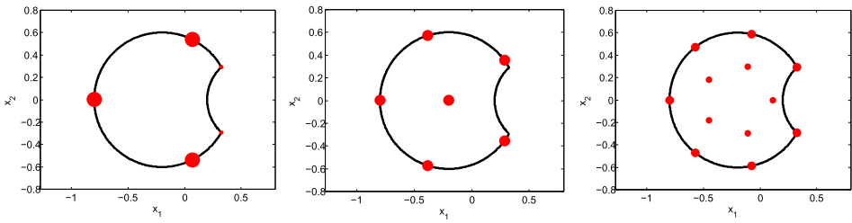
FIG. 5. The polygon (bold black) of Example 6.4 and the support of the optimal design measure (red points) where the size of the points corresponds to the respective weights for d = 1 (left), d = 2 (middle), d = 3 (right) and \delta = 3 .
