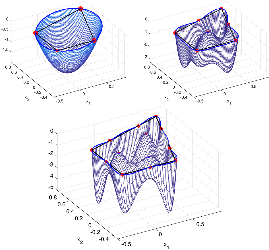
FIG. 3. The polynomial p_d^* - \binom{2+d}{2} where p_d^* denotes the Christoffel polynomial of Example 6.2 for d = 1 (top left), d = 2 (top right), d = 3 (bottom middle). The red points correspond to the \binom{2+d}{2} -level set of the Christoffel polynomial.
