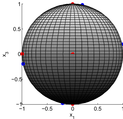
FIG. 8. Support points recovered in Example 6.6 for the D -optimal design and d = 1 (red) and the points which are recovered when additionally fixing some moments as described in Section 6.7 (blue).
