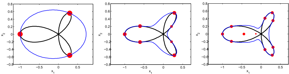
FIG. 6. The polygon (bold black) of Example 6.5, the support of the optimal design measure (red points) where the size of the points corresponds to the respective weights, and the \binom{2+d}{2} -level set of the Christoffel polynomial (thin blue) for d = 1 (left), d = 2 (middle), d = 3 (right) and \delta = 3 .
