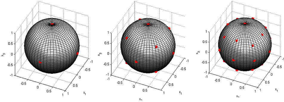
FIG. 7. The red points illustrate the support of the optimal design measure for d = 1 (left), d = 2 (middle), d = 3 (right) and \delta = 0 for Example 6.6.
