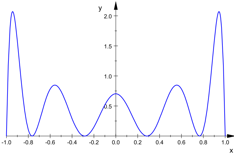
FIG. 1. Polynomial p^* for Example 6.1.
