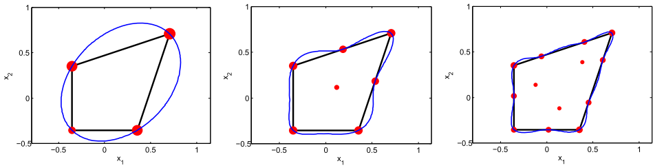
FIG. 2. The polygon (bold black) of Example 6.2, the support of the optimal design measure (red points) where the size of the points corresponds to the respective weights, and the \binom{2+d}{2} -level set of the Christoffel polynomial (thin blue) for d = 1 (left), d = 2 (middle), d = 3 (right) and \delta = 3 .
