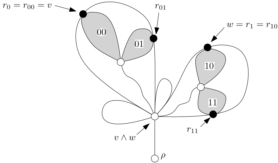
Fig. 3. Part of a routing for a pair v, w of points of C . The pair (r_{01}, r_{11}) is a signpost for (v, w) . For each b \in \{0, 1\}^2 , we must have r_{b0} = r_b , and r_{b1} must lie within the grey subtree labelled with b .
