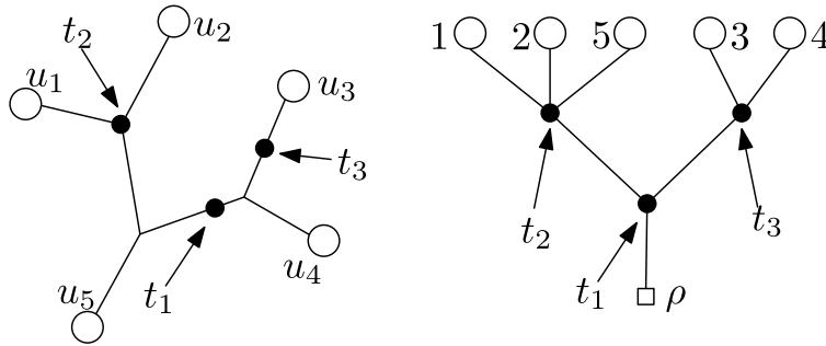
Fig. 2. Left: the subtree of T spanned by vertices u_1, \dots, u_5 . Cuts on this subtree arrive at times t_1 < t_2 < t_3 . Right: the resulting genealogical tree F with leaves 1, \dots, 5 . The figure indicates the correspondence between cuts and branchpoints of F .
