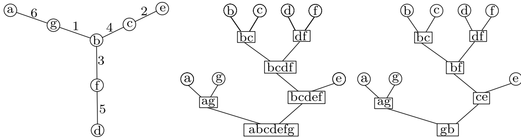
Fig. 1. Left: A discrete tree T with vertex labels from \{a, b, c, d, e, f, g\} . Edges are marked with the time at which they are cut. Center: The resulting cut tree C . Each internal vertex corresponds to a cut, and is labelled by the block of the fragmentation process which is split by that cut. Right: Cuts correspond to edges in T ; here each internal vertex of C is labelled by the pair of endpoints of the corresponding edge.
