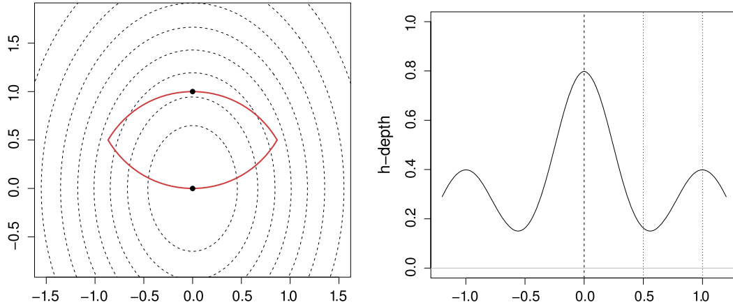
FIG. 1. Left: Some contours of D_T of a centred bivariate Gaussian distribution P (dashed), the point maximizing the depth z = (0, 0) , and x = (0, 1) . The set R(x, z) is the area inside the solid curve passing through x and z . The points in R(x, z) far from x and z attain lower depth values than D(x, P) , meaning that P-3 is not satisfied for D_T . Right: Depth D_h of an atomic distribution P in \mathbb{R} supported in three points z = 0, x_1 = 1 and x_2 = -1 . Here, z is the expectation of X \sim P , and the sole maximizer of D_h over \mathbb{R} . The set R(x_1, z) is the interval (z, x_1) . We see that D_h(1/2, P) < D_h(x_1, P) , meaning that D_h satisfies neither ZS-3, nor P-3.
