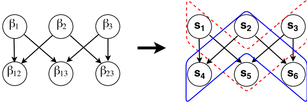
FIG. 1. Left: A DAG \mathcal{D} for a two-way interaction model with three predictors. In HSM, the DAG \mathcal{D} encodes the sparsity structure: a node's parameters must be set to zero if it has a parent with zeroed parameters. Right: The same \mathcal{D} specified using our notation: each node contains only one element and the correspondence between s_i and \beta_j is as shown. In red dashed contour, \text{ancestors}(\mathcal{D}; s_5) = \{s_1, s_3, s_5\} include both main effects, \beta_1 and \beta_3 , in the ancestor group of the interaction effect \beta_{13} . In blue solid contour, \text{descendants}(\mathcal{D}; s_2) = \{s_2, s_4, s_6\} contains both interaction effects involving main effect \beta_2 .
