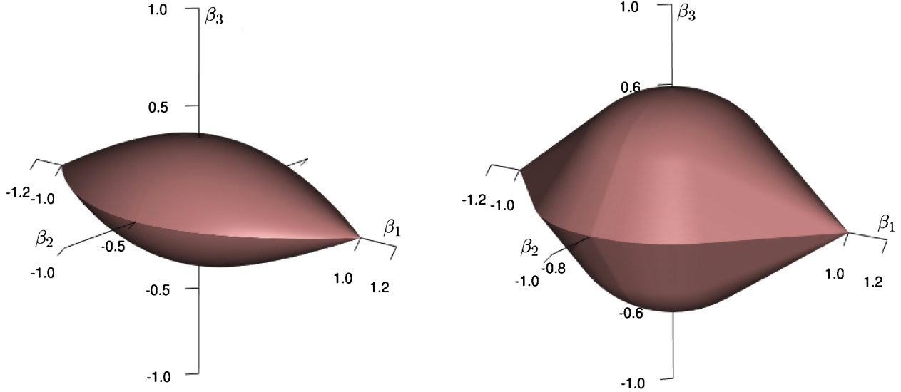
FIG. 3. For \beta \in \mathbb{R}^3 and the DAG \{1\} \rightarrow \{2\} \rightarrow \{3\} , left: the unit ball of \Omega_{GL}^{d(\mathcal{D})}(\beta; w) where d(\mathcal{D}) = \{\{1, 2, 3\}, \{2, 3\}, \{3\}\} and w = (1, 1, 1) , and right: the unit ball of \Omega_{LOG}^{a(\mathcal{D})}(\beta; w) where a(\mathcal{D}) = \{\{1\}, \{1, 2\}, \{1, 2, 3\}\} and w = (1, \sqrt{2}, \sqrt{3}) .
