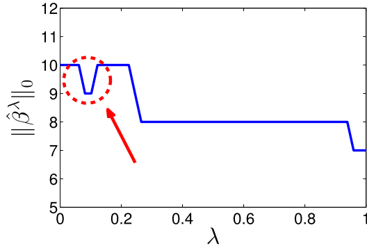
FIG. 2. The number of active elements in the LASSO's solution as a function of \lambda . The size of the active set at one location grows as we increase \lambda , and hence this function does not match the intuition. For the details of this experiment, see the supplementary material [29].
