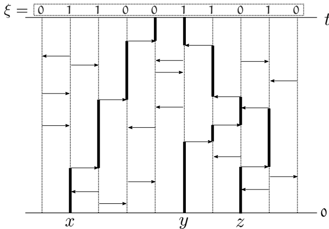
FIG. 1. Illustration of the system of coalescing random walks to which the voter model is dual. The horizontal axis represents space (which is one-dimensional in this picture) and the vertical axis represents time; arrows are plotted as described in the text. On top, a configuration \xi \in \{0, 1\}^{\mathbb{Z}^d} is represented. The thick vertical paths represent the trajectories of (Y_s^x) , (Y_s^y) , (Y_s^z) for 0 \leq s \leq t . In the situation illustrated, we have \xi(Y_t^x) = 0 and \xi(Y_t^y) = \xi(Y_t^z) = 1 .
