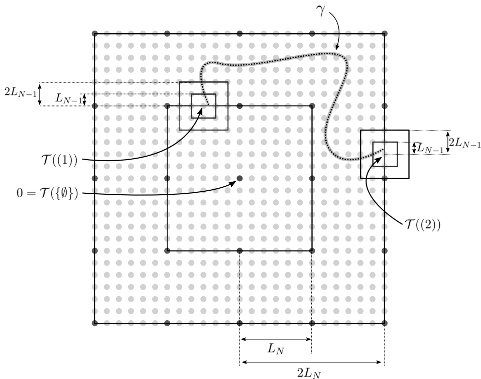
FIG. 2. Illustration of the relation between the proper embedding \mathcal{T} (see Definition 4.2) and the path \gamma that appears in Lemma 4.4. The light grey circles and dark grey circles represent points of the lattices \mathcal{L}_{N-1} and \mathcal{L}_N , respectively.
