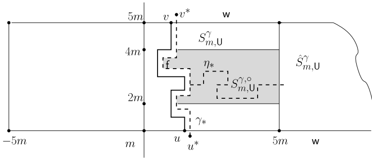
FIG. 2. The dual path \gamma_* = \gamma_*^{u,v} . Event \mathcal{D}^\circ : a dual path \eta_* crosses from left to right the middle section S_{m,U}^{\gamma,\circ} of S_{m,U}^\gamma and, as such, rules out the occurrence of the event \mathcal{R}_k . The boundary conditions (for the direct model) on the semi-infinite strip \hat{S}_{m,U}^\gamma are w on the upper and lower parts, and f on \gamma_* .
