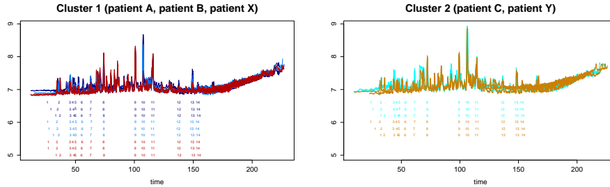
FIG 6. Total alignment obtained by block k -mean alignment, considering k = 2 clusters. The two clusters are represented in two different panels.
