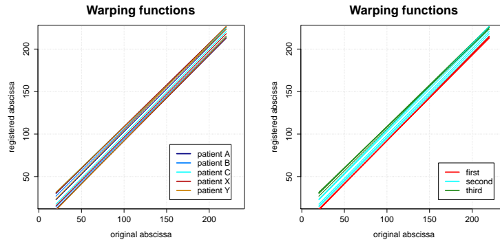
FIG 5. Total warping functions for the case k = 1 colored according to the patient (left panel) and to the order of the TIC profile within the patient (right panel).
