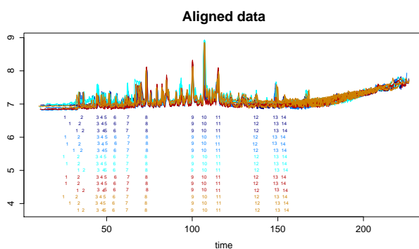
FIG 4. Total alignment obtained by block k -mean alignment, considering k = 1 cluster (simple alignment without clustering).
