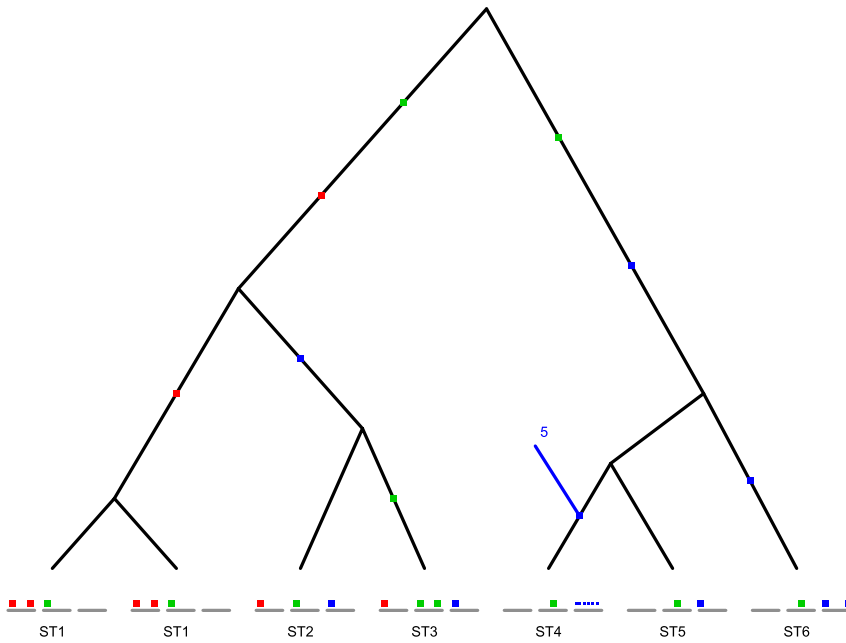
FIG. 2. Example clonal frame and resulting data set for 7 isolates at 3 loci. Mutations are denoted by squares, and the color denotes the locus that the mutation occurs on. There is a single recombination event, denoted by a square labeled with the number of differences to the ancestral sequence that event introduces. For this example, there are 6 distinct sequence types, denoted ST1 to ST6. We have an SLV pair at locus 2 (ST2 and ST3) and 3 SLV pairs at locus 3 (all distinct pairs of ST4 to ST6).
