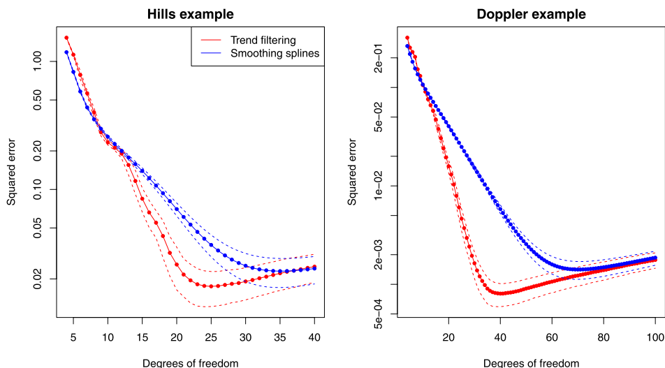
FIG. 6. Shown is the squared error loss in predicting the true function f_0 , averaged over the input points, for the hills data example on the left, and the Doppler example on the right. In each setup, trend filtering and smoothing spline estimators were fit over a range of degrees of freedom values; the red curves display the loss for trend filtering, and the blue curves for smoothing splines. The results were averaged over 50 simulated data sets, and the standard deviations are denoted by dotted lines. In these examples, trend filtering has a generally better predictive accuracy than smoothing splines, especially for models of low to intermediate complexity (degrees of freedom).
