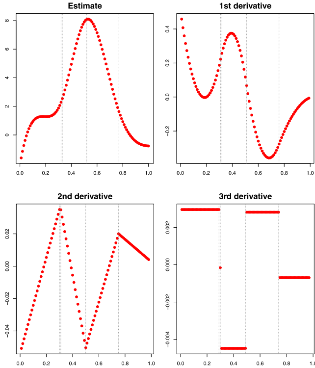
FIG. 3. The leftmost panel shows the same cubic trend filtering estimate as in Figure 2 (but here we do not use linear interpolation to emphasize the discrete nature of the estimate). The components of this estimate appear to be the evaluations of a continuous piecewise polynomial function. Moreover, its discrete 1st and 2nd derivatives (given by multiplying by D^{(1)} and D^{(2)} , resp.) also appear to be continuous, and its discrete third derivative (from multiplication by D^{(3)} ) is piecewise constant within each interval. Hence, we might believe that such a trend filtering estimate actually represents the evaluations of a 3rd degree spline over the inputs x_i = i/n , i = 1, \dots, n . We address this idea in Section 4.
