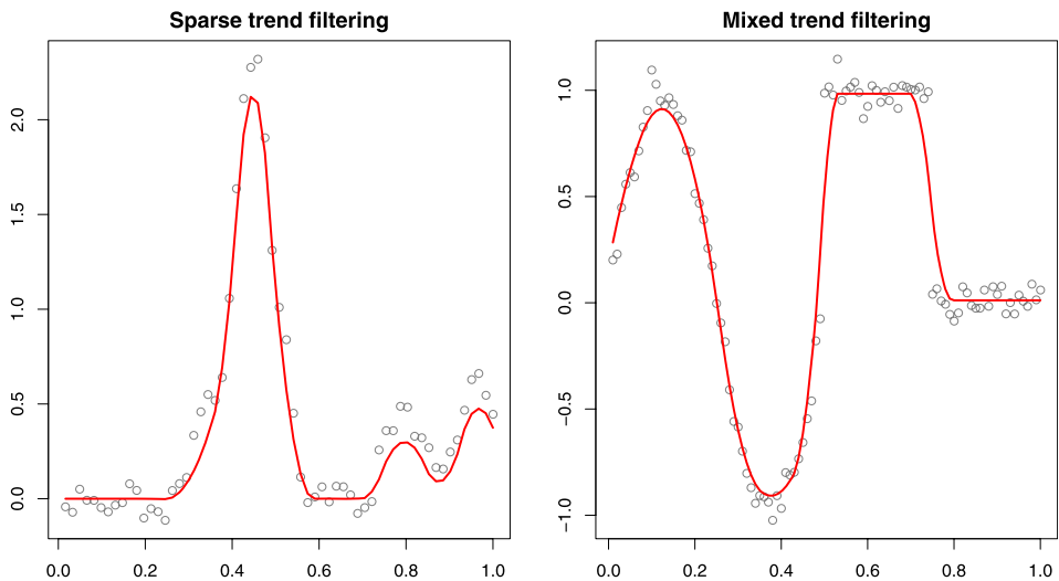
FIG. 11. Left panel: a small example of sparse quadratic trend filtering ( k = 2 ). The estimate \hat{\beta} in (43) is identically zero for inputs approximately between 0 and 0.25, and 0.6 and 0.75. Right panel: an example of constant/quadratic mixed trend filtering ( k_1 = 0 and k_2 = 2 ). The estimate defined in (44) is first piecewise quadratic over the first half of its domain, but then is flat in two stretches over the second half.
