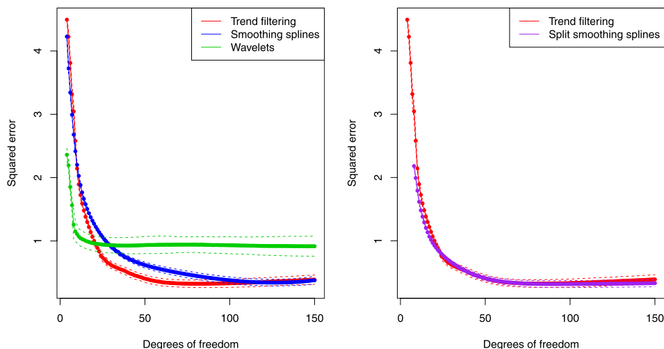
FIG. 10. Left plot: the squared error loss in estimating the true light curve for the quasar spectrum data, using trend filtering, smoothing splines and wavelets, fit over a range of model complexities (degrees of freedom values). The results were averaged over 20 simulated data sets, with standard errors drawn as dotted lines. Trend filtering achieves a significantly lower squared error loss than smoothing splines for models of low complexity; both perform much better than wavelets. Right plot: trend filtering versus a smoothing spline estimator that fits a different smoothing parameter on two halves of the domains (on either side of the peak around x = 3.6 ); the methods perform comparably.
