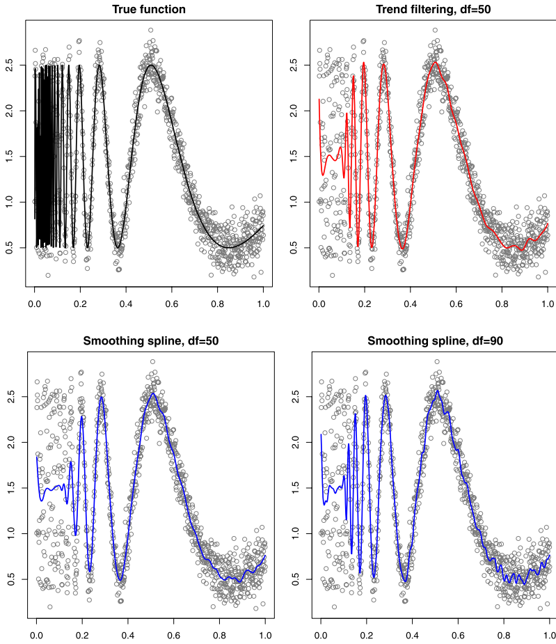
FIG. 5. An example with n = 1000 noisy observations of the Doppler function, f(x) = \sin(4/x) + 1.5 , drawn in the top left panel. The top right and bottom left panels show the cubic trend filtering and smoothing spline estimates, each with 50 degrees of freedom; the former captures approximately 4 cycles of the Doppler function, and the latter only 3. If we nearly double the model complexity, namely, we use 90 degrees of freedom, then the smoothing spline estimate is finally able to capture 4 cycles, but the estimate now becomes very jagged on the right-hand side of the plot.
