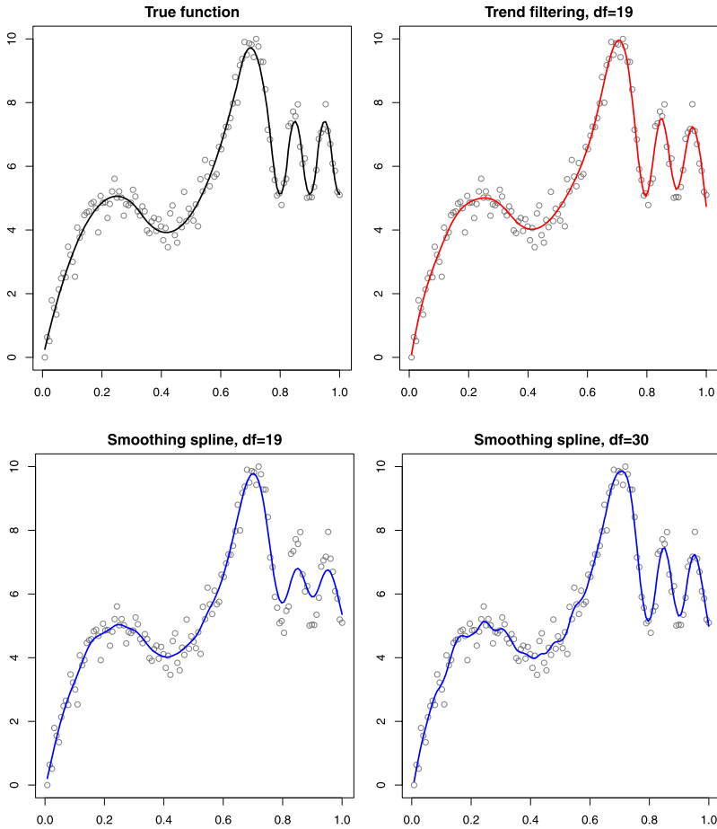
FIG. 4. An example with n = 128 observations drawn from a model where the underlying function has variable spatial smoothness, as shown in the top left panel. The cubic trend filtering estimate with 19 degrees of freedom, shown in the top right panel, picks up the appropriate level of smoothness at different spatial locations: smooth at the left-hand side of the domain, and wiggly at the right-hand side. When also allowed 19 degrees of freedom, the cubic smoothing spline estimate in the bottom left panel grossly underestimates the signal on the right-hand side of the domain. The bottom right panel shows the smooth spline estimate with 30 degrees of freedom, tuned so that it displays the appropriate level of adaptivity on the right-hand side; but now, it is overly adaptive on the left-hand side.
