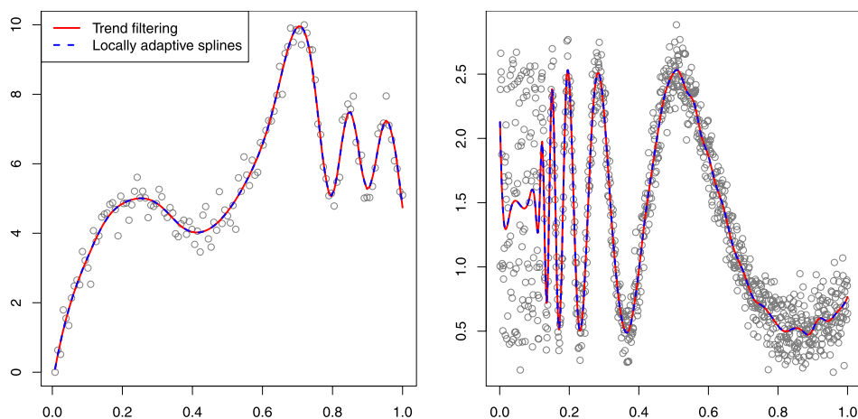
FIG. 7. Trend filtering and locally adaptive regression spline estimates, using the same values of the tuning parameter \lambda , for the hills and Doppler data examples considered in Section 2.2. The trend filtering estimates are drawn as solid red lines, and locally adaptive regression splines as dotted blue lines; in both examples, the two estimates are basically indistinguishable by eye.
