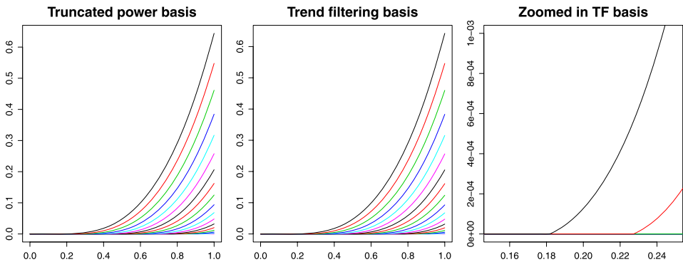
FIG. 8. For n = 22 inputs (evenly spaced over [0, 1] ) and k = 3 , the left panel shows the truncated power basis functions in (19) and the center panel shows the basis functions in (25) utilized by trend filtering. The two sets of basis functions appear very similar. The right plot is a zoomed in version of the center plot, and shows the nonsmooth nature of the trend filtering basis functions—here (for k = 3 ) they have discontinuous first and second derivatives.
