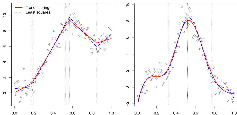
FIG. 2. Examples of the shrinkage effect for linear trend filtering ( k = 1 , left panel) and for cubic trend filtering ( k = 3 , right panel). In each panel, the solid red line is the trend filtering estimate (at a particular value of \lambda ), and the dashed blue line is the regression spline estimate of the same order and with the same knots, with the vertical lines marking the locations of the knots. The trend filtering estimates on the left and right have shrunk 1st and 3rd derivatives, respectively, compared to their regression spline counterparts.
