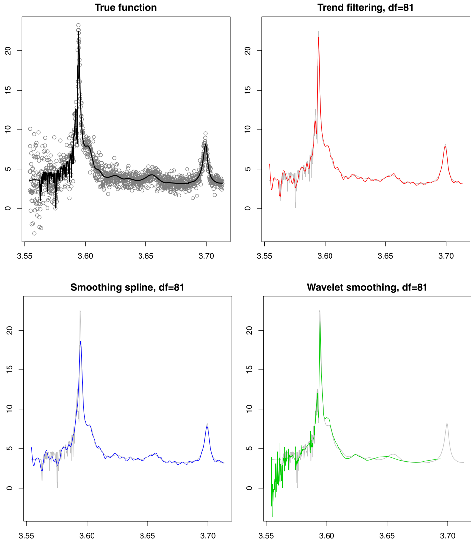
FIG. 9. The top left panel shows data simulated from a model for quasar spectrum. The true curve, in black, displays flux as a function of log wavelength. The gray points are noisy observations at n = 1172 wavelength values. We fit trend filtering, smoothing splines, and wavelets to these points, and tuned each to have 81 degrees of freedom. (This value was chosen because it corresponded to the trend filtering model with the minimum squared error loss, averaged 20 simulations—see Figure 10.) The resulting estimates are displayed in the top right, bottom left and bottom right panels, respectively (with the true function plotted in the background, in gray). Trend filtering and smoothing splines give similar fits, except that trend filtering does a better job of estimating the large peak at around x = 3.6 , as well as some of the finer features of the true function to the left of this. Wavelet smoothing also does well in detecting the extreme peak, but then overfits the true function on the left-hand side, and underfits on the right.
