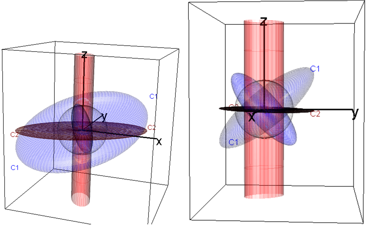
FIG. A.1. Two views of an example of generalized ellipsoids. \mathbf{C}_1 (blue) determines a proper, fat ellipsoid; its inverse \mathbf{C}_1^{-1} also generates a proper ellipsoid. \mathbf{C}_2 (red) determines an improper, flat ellipsoid, whose inverse \mathbf{C}_2^{-1} is an unbounded cylinder of elliptical cross section. The scale of these images is defined by a unit sphere (gray). The left panel shows that \mathbf{C}_2 is a projection of \mathbf{C}_1 onto the plane where z = 0 . The right panel shows a view illustrating the orthogonality of each \mathbf{C} and its dual, \mathbf{C}^{-1} .
