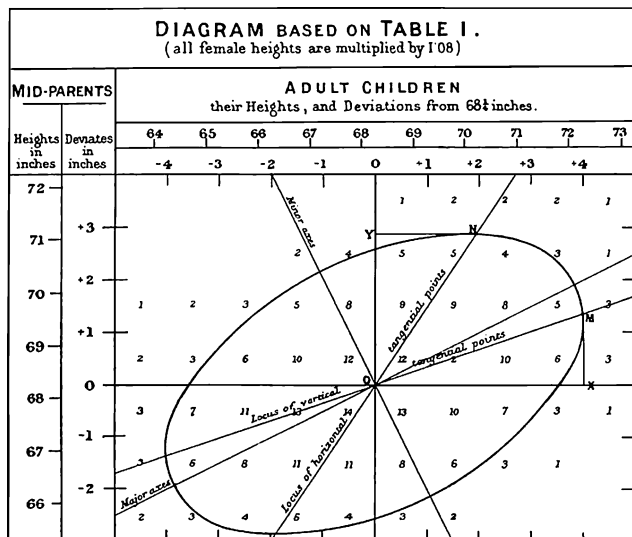
FIG. 1. Galton's 1886 diagram, showing the relationship of height of children to the average of their parents' height. The diagram is essentially an overlay of a geometrical interpretation on a bivariate grouped frequency distribution, shown as numbers.
