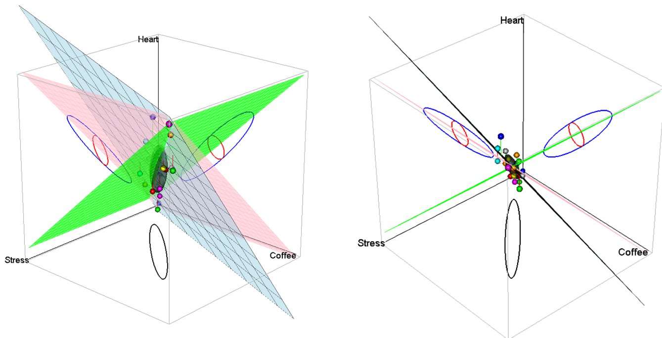
FIG. 17. 3D views of the relationship between Heart, Coffee and Stress, showing the three regression planes for the marginal models, Heart \sim Coffee (green), Heart \sim Stress (pink), and the joint model, Heart \sim Coffee + Stress (light blue). Left: a standard view; right: a view showing all three regression planes on edge. The ellipses in the side panels are 2D projections of the standard conditional (red) and marginal (blue) ellipsoids, as shown in Figure 18.
