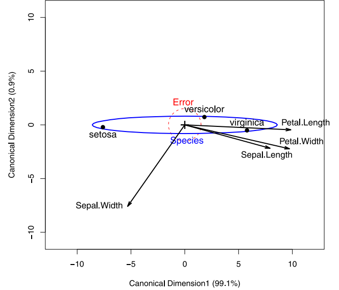
FIG. 22. Canonical HE plot for the Iris data. In this plot, the \mathbf{H} ellipse is shown using effect-size scaling to preserve resolution, and the variable vectors have been multiplied by a constant to approximately fill the plot space. The projections of the variable vectors on the coordinate axes show the correlations of the variables with the canonical dimensions.
