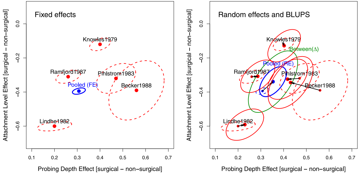
FIG. 29. Multivariate meta-analysis visualizations for five periodontal treatment studies with outcome measures PD and AL. Left: Individual study estimates \mathbf{y}_i and 40% standard ellipses for \mathbf{S}_i (dashed, red) together with the pooled, fixed effects estimate and its associated covariance ellipse (blue). Right: BLUPs from the random-effects multivariate meta-analysis model and their associated covariance ellipses (red, solid), together with the pooled, population-averaged estimate and its covariance ellipse (blue), and the estimate of the between-study covariance matrix, \boldsymbol{\Delta} (green). Arrows show the differences between the FE and the RE models.
