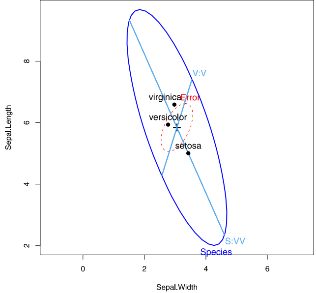
FIG. 21. \mathbf{H} and \mathbf{E} matrices for sepal width and sepal length in the iris data, together with \mathbf{H} matrices for testing two orthogonal contrasts in the species effect.
