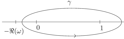
FIG. 1. Possible integration contour.
