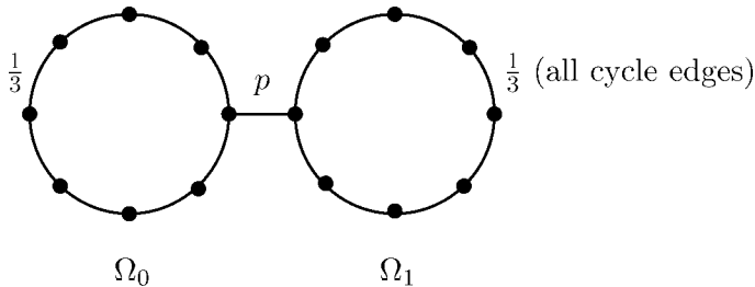
FIG. 1. Pince-nez graph ( n = 8 ).
