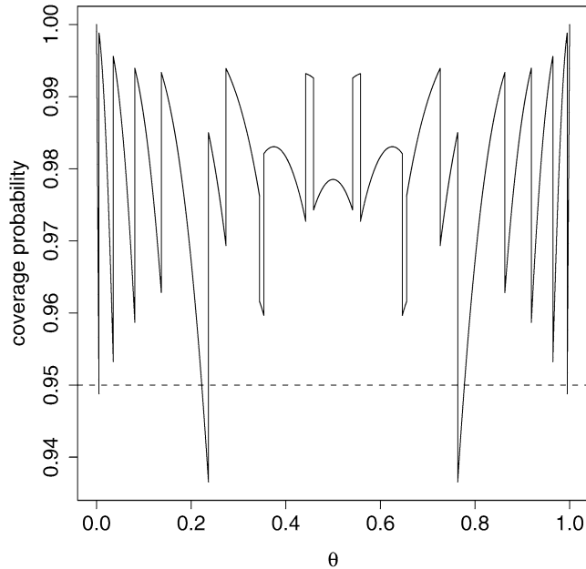
FIG. 1. Coverage probability of the nominal 95% confidence interval for the binomial distribution with sample size n = 10 calculated by the function prop.test in the R statistical computing language (R Development Core Team, 2004). This is the Wilson (also called, score) interval with continuity correction and modifications when x = 0 or x = n . The dashed line is the nominal level. The solid line is the coverage probability of the interval as a function of the success probability \theta .
