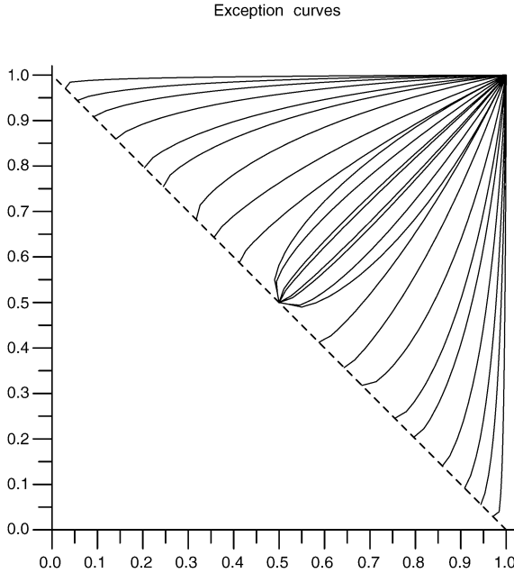
FIG. 1. Some of the curves satisfying (3.22).
