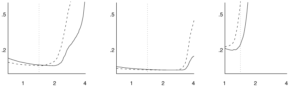
FIG. 1. The average of 1000 simulated ME of the MC+ (solid) and SCAD (dashed) as functions of \lambda/\sqrt{(\log p)/n} for (n, p, d^0, \beta_*, \gamma) = (50, 12, 3, 1.5, 3.7), (100, 12, 3, 1.5, 3.7) and (100, 300, 15, 1, 2.5) , from the left, with dotted vertical at \lambda = \sqrt{2(\log p)/n} .
