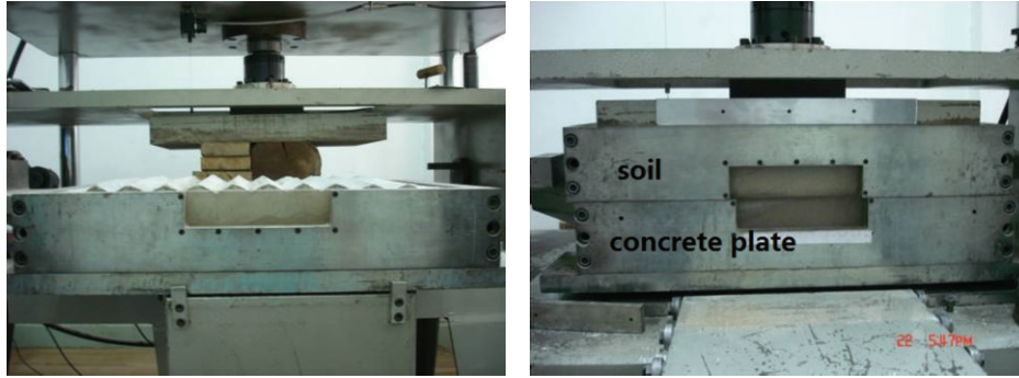
FIGURE 2: Setup of the specimen box.
