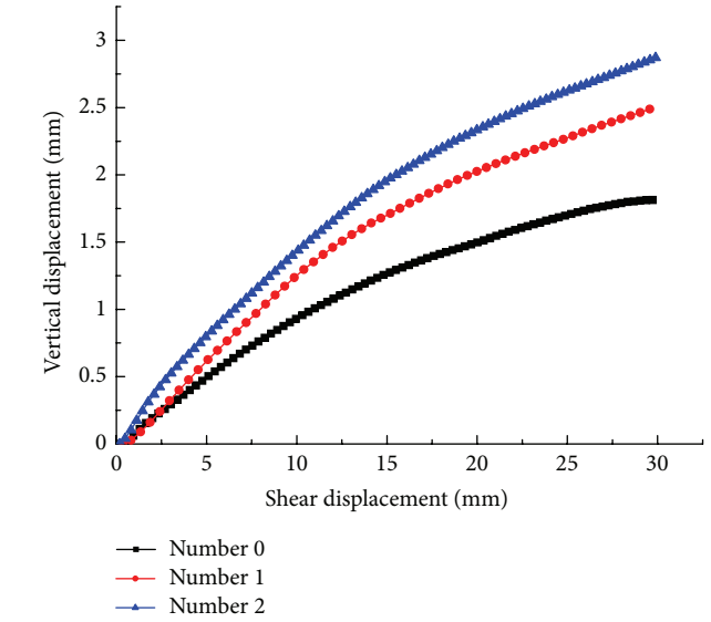
FIGURE 11: The vertical dilative displacement for interfaces of different roughness.
