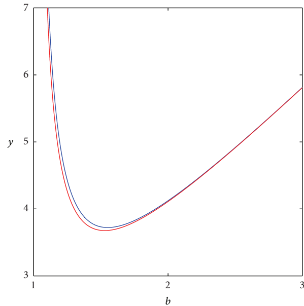
FIGURE 4: This graph shows the average of the attracting 2-cycle (blue color) in contrast with the equilibrium that results from constant stoking equals the average of h_0 and h_1 , where h_0 = b + 1/(b - 1) and h_1 = b .
