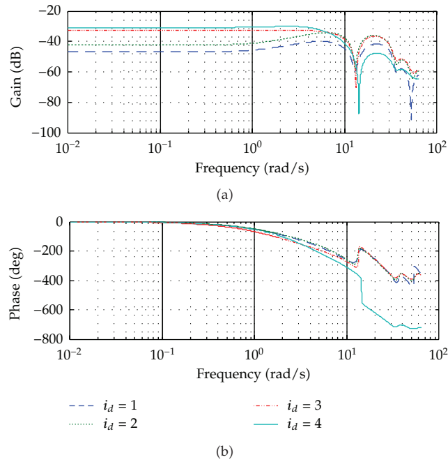
Figure 4: Bode plots of the the feedback controllers K^{i_d}(z) 's ( n = 8 ).
