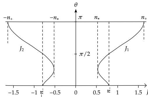
Figure 13: Curve of intermediate states (5.10) in (J, \theta) -plane.
