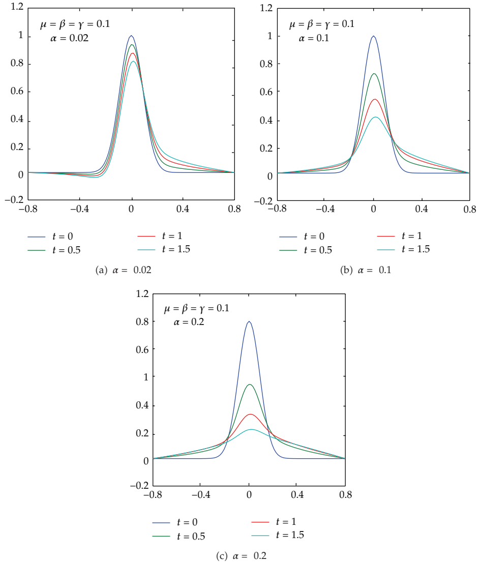
Figure 1: The evolution of u(x,t) with different \alpha .
