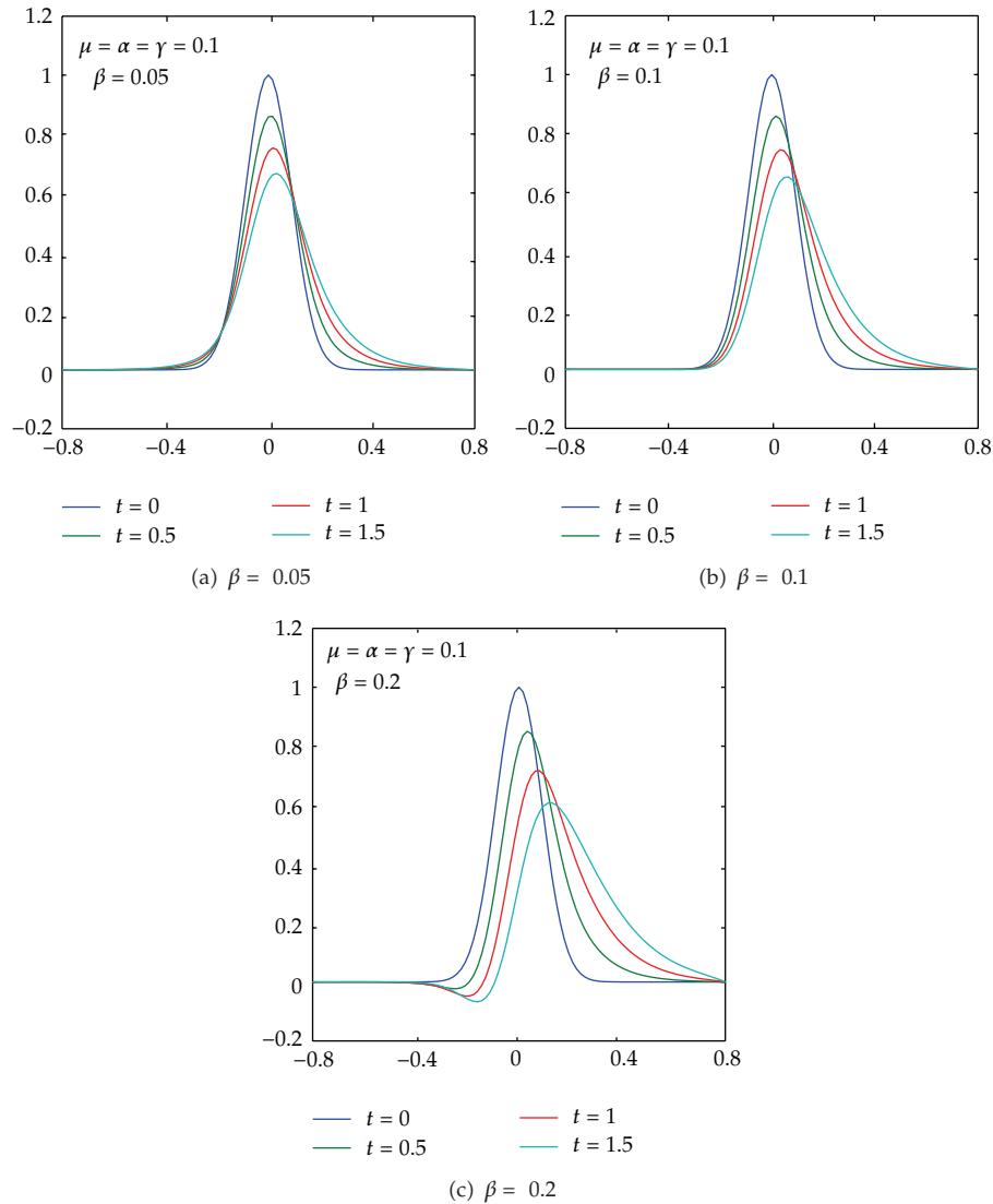
Figure 2: The evolution of u(x,t) with different \beta .
