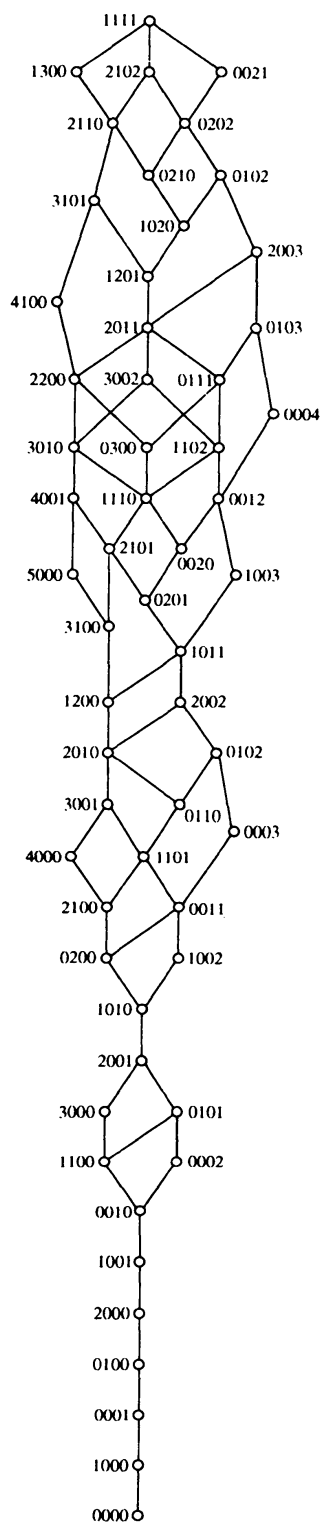
FIGURE IV: The partial ordering of \Lambda^+(\rho) in F_4 .
