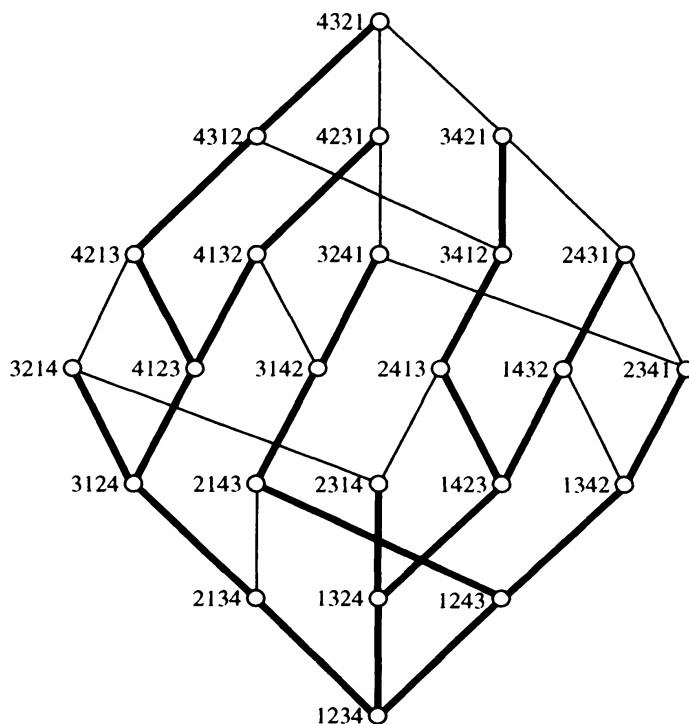
FIGURE III: The weak ordering of A_3 .
