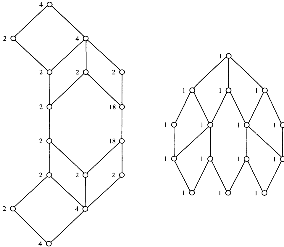
FIGURES I AND II: The posets corresponding to the conjugacy classes of s_2s_3s_2s_3s_4 in F_4 and s_1s_3 in A_4 .
