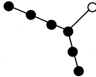
Fig. 6. Plumbing graph for the (2, 3, 4) -pretzel.
