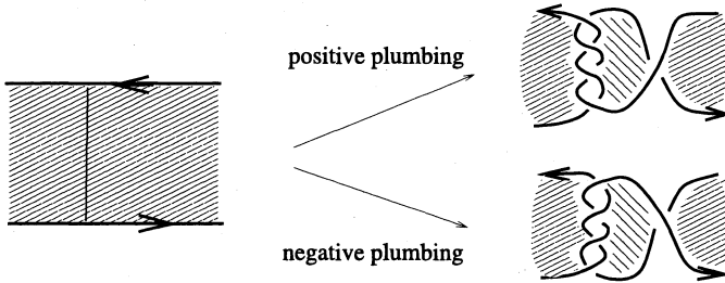
Fig. 2. Fourth iterated Hopf plumbing.
