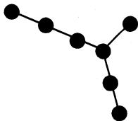
Fig. 5. The (2, 3, 4) -star graph.
