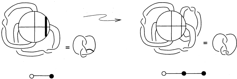
Fig. 4. Graphs and plumbing.
