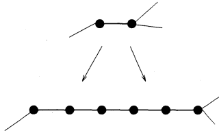
Fig. 3. Extending an edge of a graph.
