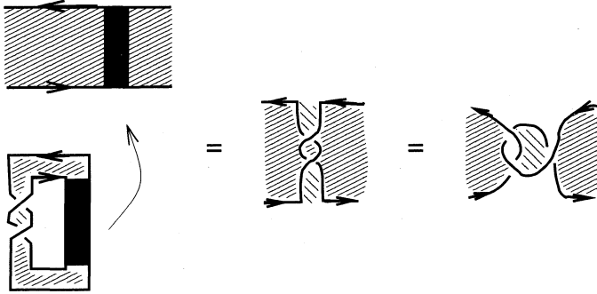
Fig. 1. Positive Hopf plumbing.
