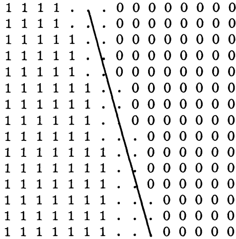
Figure 1.a ( q^* = .16 )
