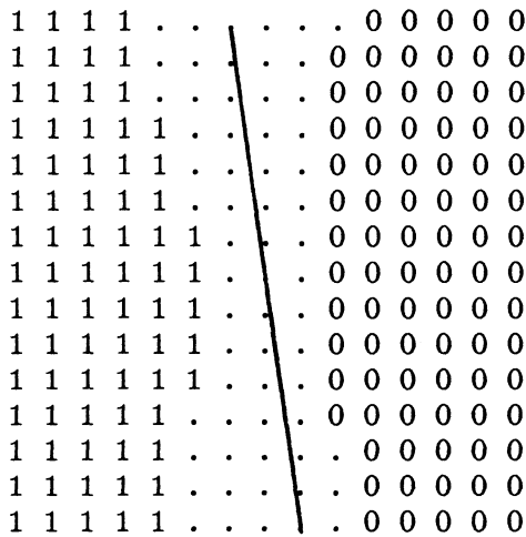
Figure 1.b ( q^* = .28 )
