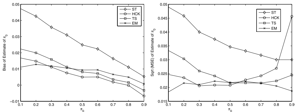
FIG 3. Bias and \sqrt{MSE} of \hat{\pi}_0 for ST, HCK, TS and EM Estimators for Normal Model (Data Generated by Normal Model with Random \delta ).
