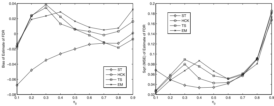
FIG 8. Bias and \sqrt{MSE} of \widehat{FDR} for ST, HCK, TS and EM Estimators for Beta Model (Data Generated by Beta Model).
