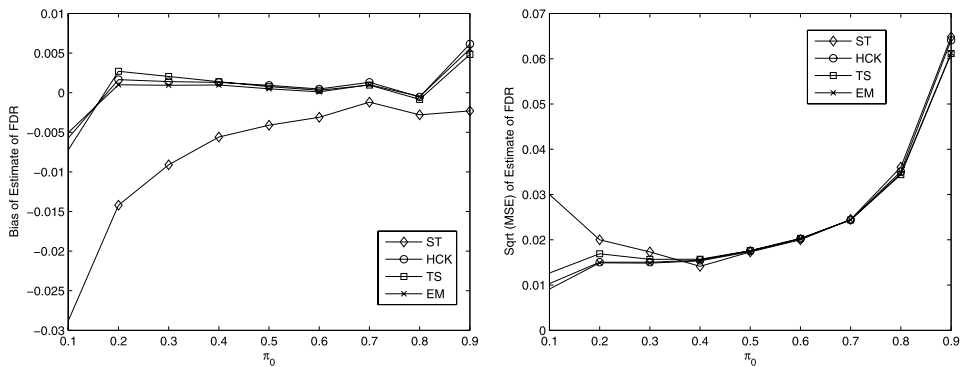
FIG 2. Bias and \sqrt{MSE} of \widehat{FDR} for ST, HCK, TS and EM Estimators for Normal Model (Data Generated by Normal Model with Fixed \delta ).
