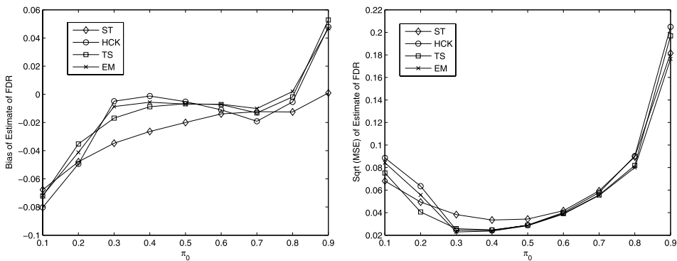
FIG 6. Bias and \sqrt{MSE} of \widehat{FDR} for ST, HCK, TS and EM Estimators for Normal Model (Data Generated by Beta Model).
