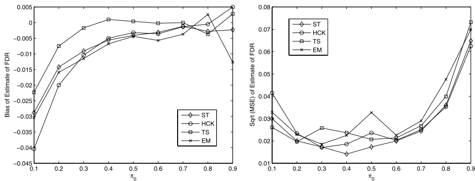
FIG 10. Bias and \sqrt{MSE} of \widehat{FDR} for ST, HCK, TS and EM Estimators for Beta Model (Data Generated by Normal Model).
