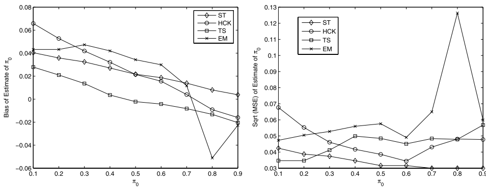
FIG 9. Bias and \sqrt{MSE} of \widehat{\pi}_0 for ST, HCK, TS and EM Estimators for Beta Model (Data Generated by Normal Model).
