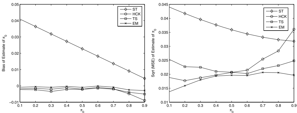
FIG 1. Bias and \sqrt{\text{MSE}} of \hat{\pi}_0 for ST, HCK, TS and EM Estimators for Normal Model (Data Generated by Normal Model with Fixed \delta ).
