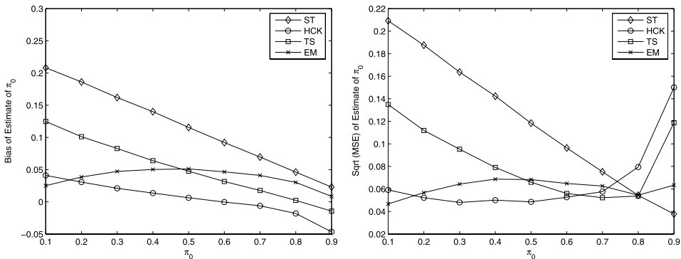
FIG 5. Bias and \sqrt{MSE} of \widehat{\pi}_0 for ST, HCK, TS and EM Estimators for Normal Model (Data Generated by Beta Model).
