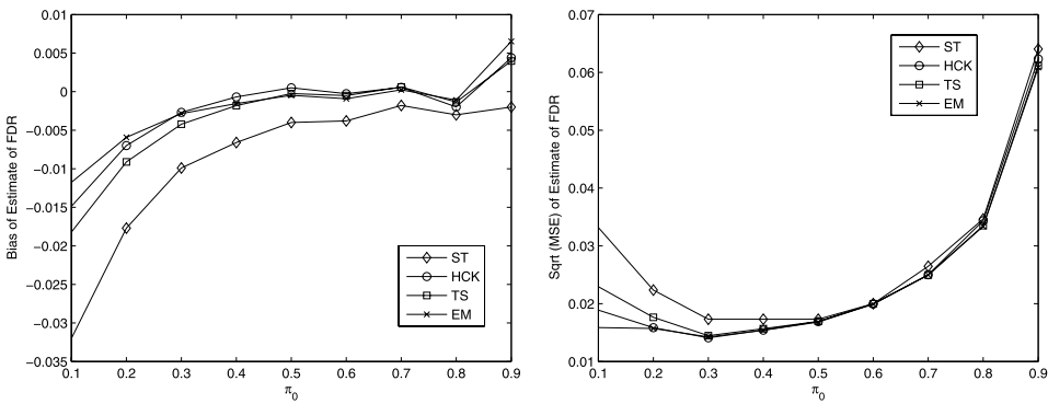
FIG 4. Bias and \sqrt{MSE} of \widehat{FDR} for ST, HCK, TS and EM Estimators for Normal Model (Data Generated by Normal Model with Random \delta ).
