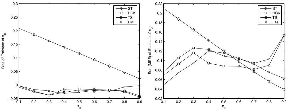
FIG 7. Bias and \sqrt{MSE} of \widehat{\pi}_0 for ST, HCK, TS and EM Estimators for Beta Model (Data Generated by Beta Model).
