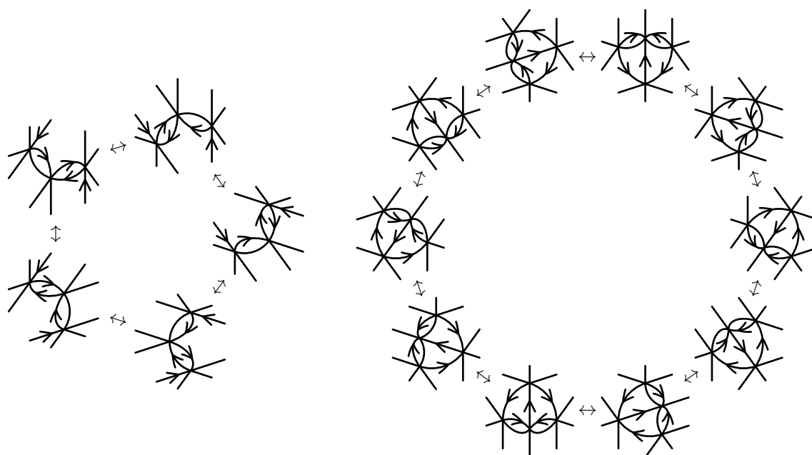
FIGURE 4. Conjectured relations between relations
