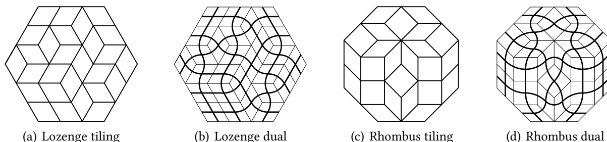
FIGURE 1. Tilings by lozenges or more general rhombuses and their duals.
