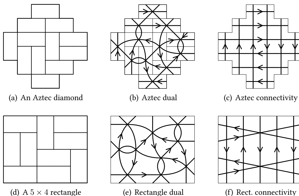
FIGURE 2. Domino tilings and their duals, along with the connectivity of the strands
