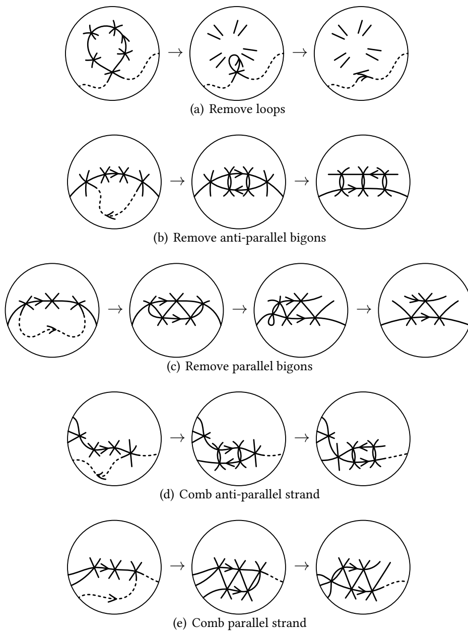
FIGURE 3. Steps in the proof of Lemma 12
