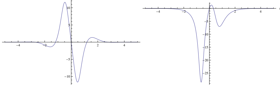
Figure 7. Plots of the density of the first integral of motion as a function of x evaluated on the stationary quadruplet soliton (70) for \alpha = \beta = \gamma = \omega = 1, \delta = 0 (left panel) and for the stationary doublet soliton (76) for \kappa = \sigma_0 = 1, \phi = 0 (right panel).
