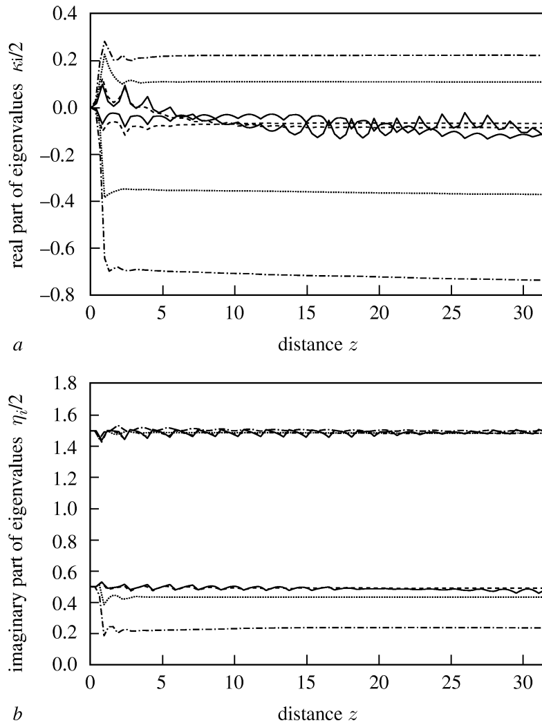
Figure 1. Spatial evolution of (a) real and (b) imaginary parts of the eigenvalues of 2\text{sech}(x) for different strengths of TOD
