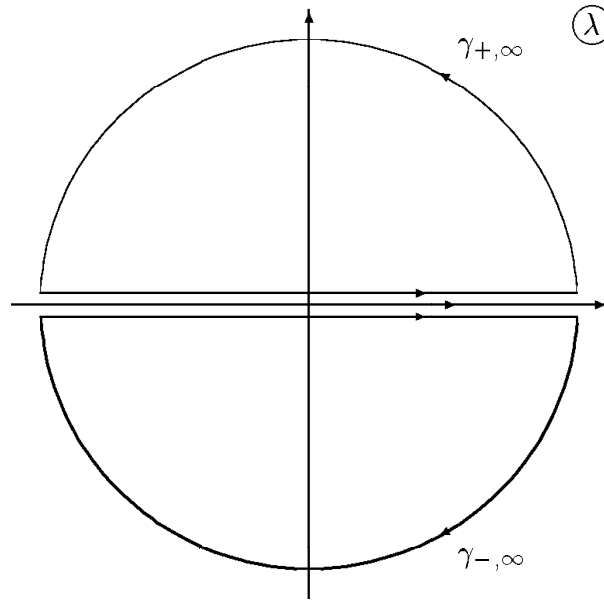
Figure 1. The contours \gamma_{\pm} = \mathbb{R} \cup \gamma_{\pm\infty} .
