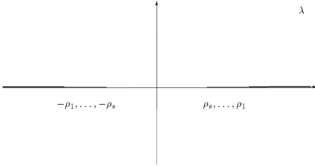
Figure 2. The continuous spectrum of the operators L_{\pm} and L .
