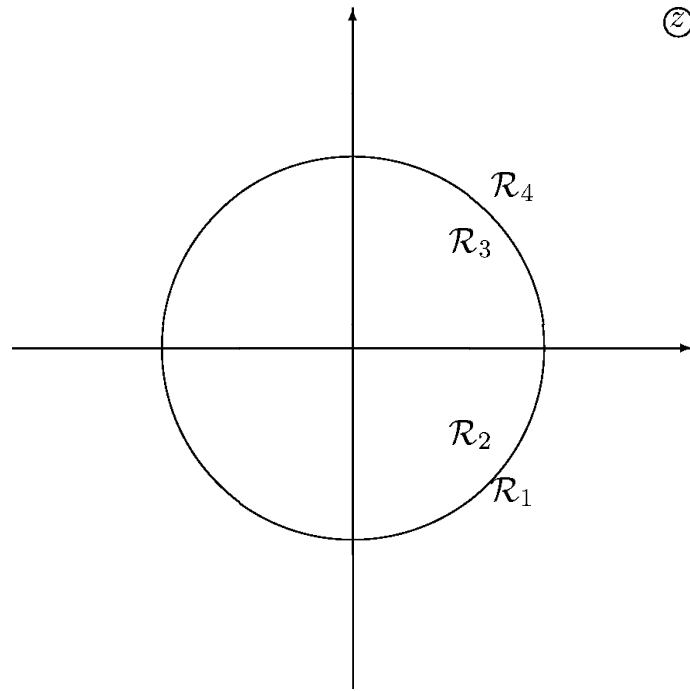
Figure 3. The continuous spectrum of L on the complex z -plane.
