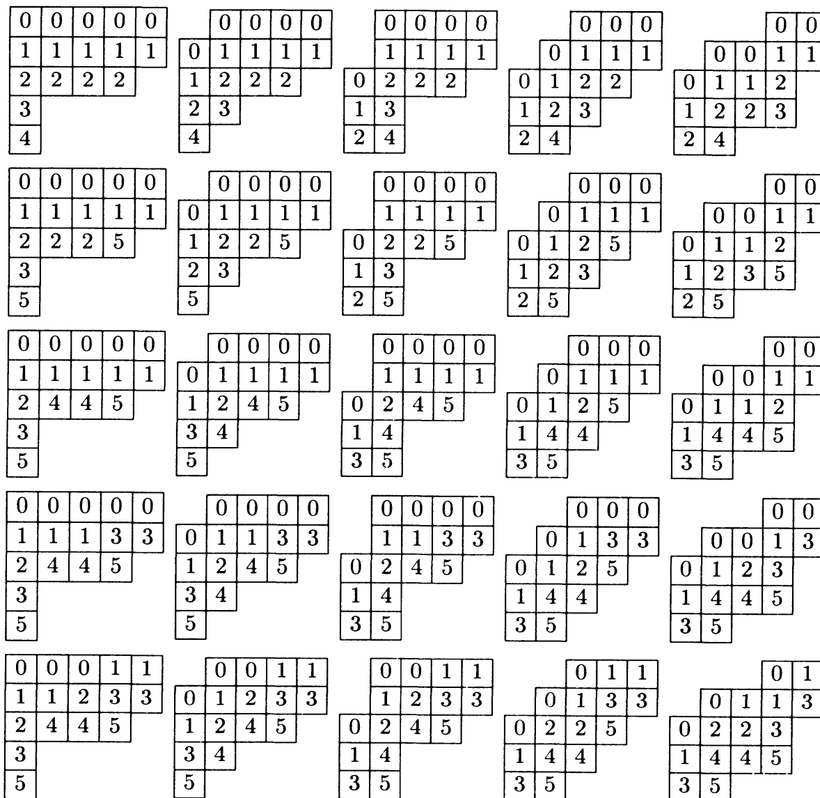
Figure 1. Commutation of jeu de taquin (right to left) and raising operations (upwards). Raising operations are grouped: e_0, e_0, e_1 ; e_2, e_1, e_2, e_1 ; e_3, e_2, e_3, e_2 ; e_4, e_4, e_3, e_2 .
