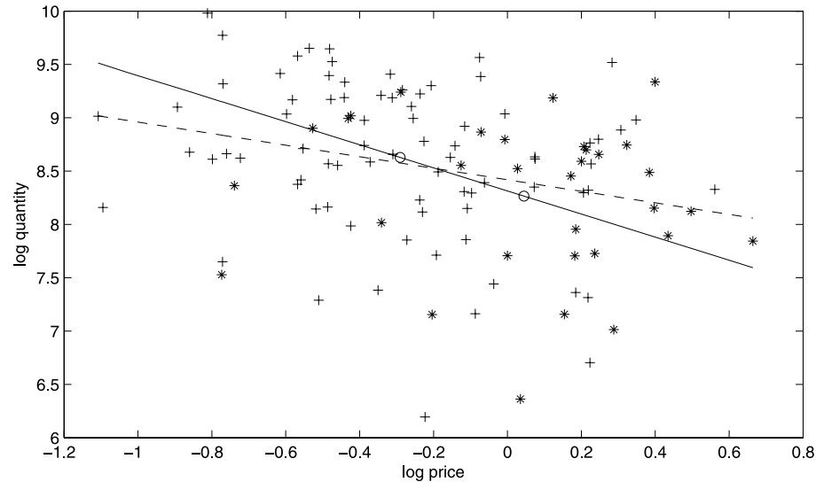
FIG. 2. Scatterplot of log prices and log quantities by weather conditions.
