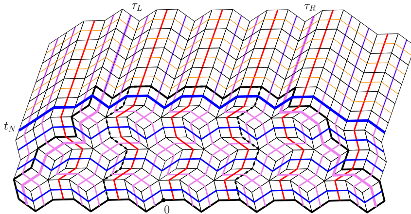
Figure 29: A graph \mathcal{D}_0 (the delimited region) and the completion \mathcal{D} – only the diamond graph is depicted. The vertical tracks ( s_i ) are red, horizontal tracks ( t_j ) blue, and the others purple. The rectangle \text{R}^{\text{hp}}(N; N) (in reality it should be wider) is delimited by dotted lines. The tracks delimiting \mathcal{D}_0 are \tau_L , \tau_R and t_N ; they are marked in bold.
