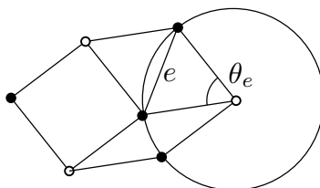
Figure 2: The edge e \in \mathbb{E} and its subtended angle \theta_e .
