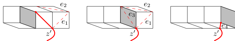
Figure 35: Three star-triangle transformations contributing to \Sigma slide the gray rhombus from left to right. If the three edges in the middle diagram are all closed, then e_4 is open with probability \frac{y_{e_1} y_{e_3}}{q} .
