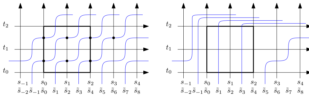
Figure 15: Left: The train tracks of a portion of a doubly-periodic isoradial graph \mathbb{G} . A grid of \mathbb{G} is given by vertical tracks (s_n) and horizontal tracks (t_n) . We denote by (\tilde{s}_n) its non-horizontal tracks. We want to make the region R(0, 2; 0, 2) have a square lattice structure by removing all the black points using star-triangle transformations. Right: The black points are removed (from the top) from the region R(0, 2; 0, 2) , making a square structure appear inside. This region contains tracks \tilde{s}_1 and \tilde{s}_3 which would be vertical in a square lattice containing R(0, 2; 0, 2) but are not vertical in the original graph \mathbb{G} on the left.
