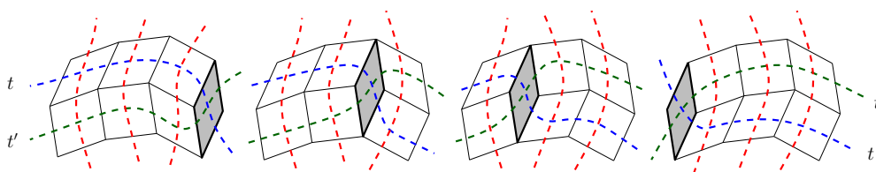
Figure 9: We move the gray rhombus from the right to the left by a sequence of star-triangle transformation. Observe that these transformations only affect the tracks t and t' , and that their ultimate effect is to exchange them.
