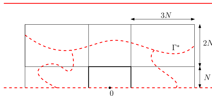
Figure 27: The strip \mathbb{S}_{4N} with wired boundary conditions on the top and free on the bottom. If \mathcal{C}_h^*(-4N, 4N; N, 3N) \cap A occurs, then \Lambda(N) is disconnected from the top of the strip. Due to the self-duality, both \mathcal{C}_h^*(-4N, 4N; N, 3N) and A conditionally on \mathcal{C}_h^*(-4N, 4N; N, 3N) occur with positive probability.
