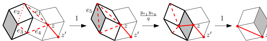
Figure 22: Three star-triangle transformations contributing to \Sigma slid the gray rhombus from left to right. The dashed edges are closed, the bold edges are open and the state of dotted edge e_2 does not really matter. The first and last passages occur with probability 1, and the second with probability y_{e_1}y_{e_4}/q .
