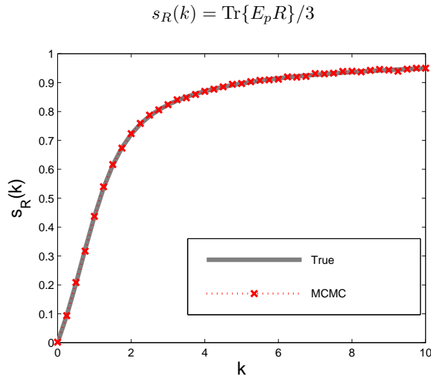
FIG. 3. MCMC estimates vs. true values (see Section 4) of s_R(k) = \text{Tr}\{E_p R\}/3 in the isotropic case \Sigma = kI .
