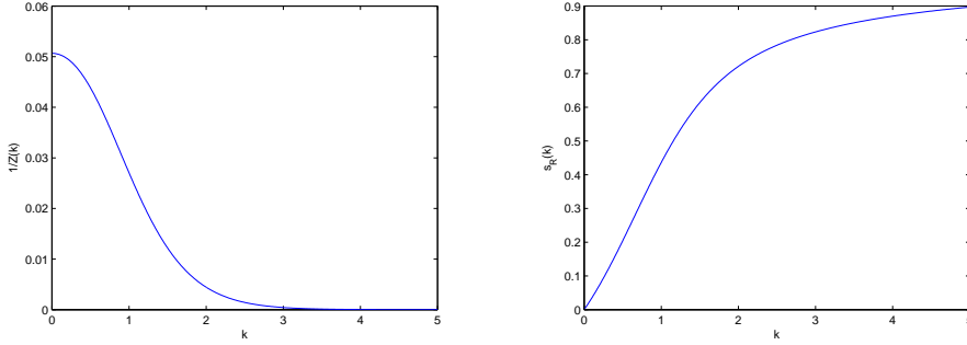
FIG. 1. Left: normalization constant \frac{1}{Z(k)} as a function of k . Right: “mean value” s_R(k) as a function of k .
