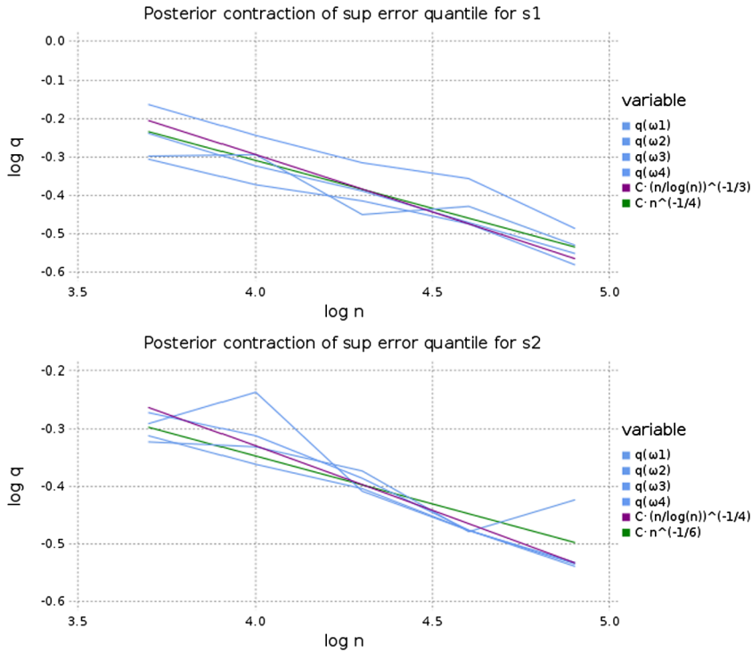
Figure 8 Estimate of the contraction rate of the size of L_\infty -balls around s covering 90% of posterior probability mass by sampling (blue); compared with likely rate (purple) and rate of Theorem 2 (green). Top: Lipschitz continuous case, example s_1 . Bottom: Hölder coefficient essentially \frac{1}{2} , example s_2 .
