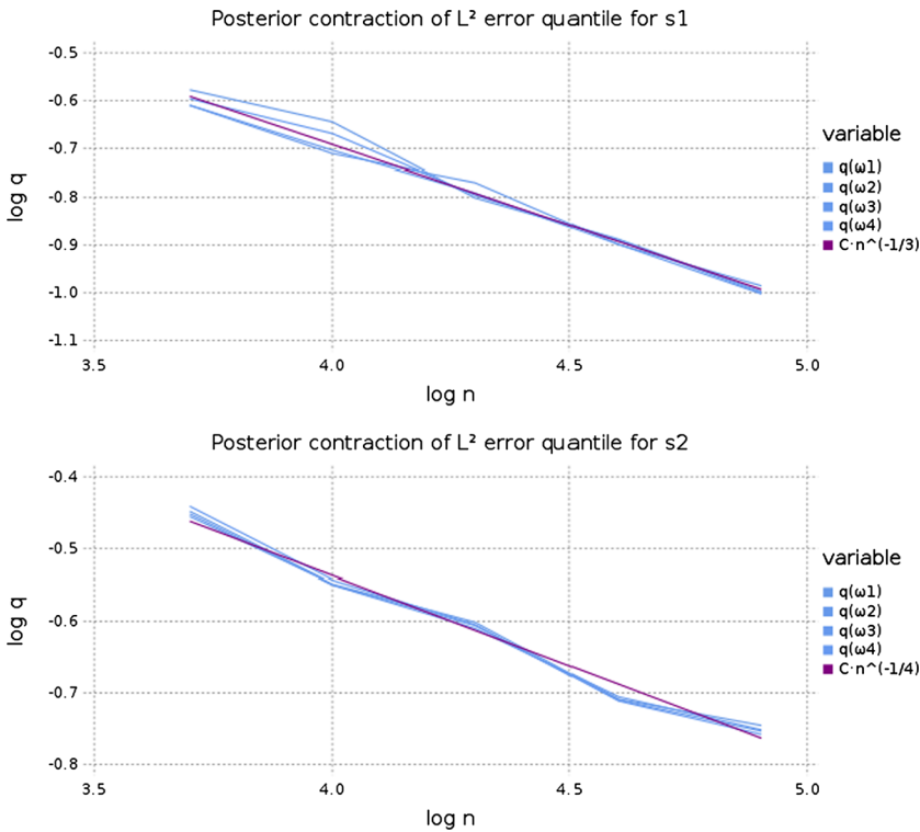
Figure 7 Estimate of the contraction rate of the size of L_2 -balls around s covering 90% of posterior probability mass by sampling (blue); compared with rate (purple). Top: Lipschitz continuous case, example s_1 . Bottom: Hölder coefficient essentially \frac{1}{2} , example s_2 .
