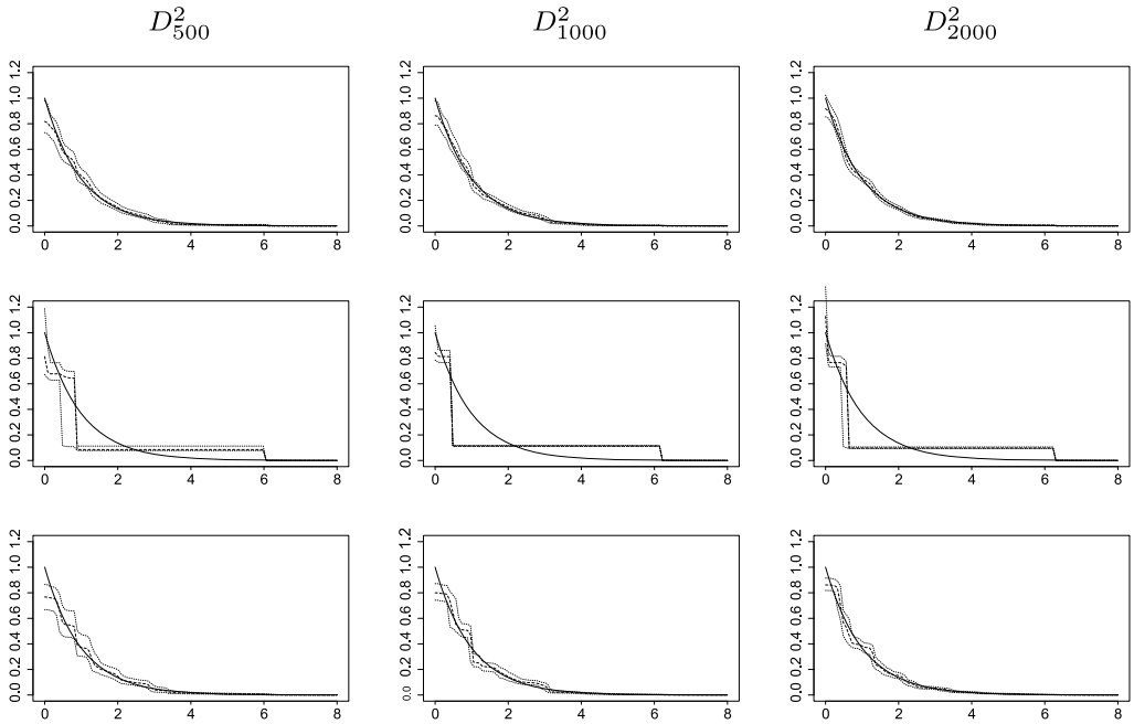
Figure 2. Estimation of \bar{\lambda}_2 from D_{500}^2 (first column), D_{1000}^2 (second column) and D_{2000}^2 (third column) using different strategies: empirical prior (row 1), fixed \gamma (row 2), hierarchical empirical prior (row 3). True density (plain line), estimate (dashed line) and confidence band (dotted lines).
