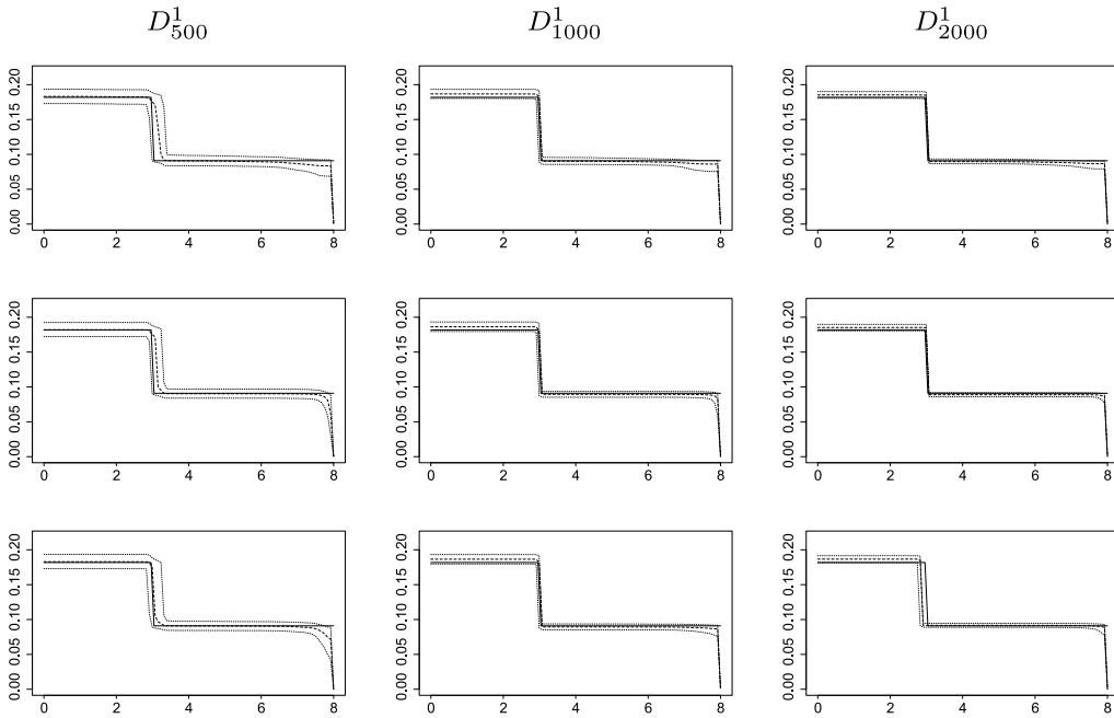
Figure 1. Estimation of \bar{\lambda}_1 from D_{500}^1 (first column), D_{1000}^1 (second column) and D_{2000}^1 (third column) using different strategies: empirical prior (row 1), fixed \gamma (row 2), hierarchical empirical prior (row 3). True density (plain line), estimate (dashed line) and confidence band (dotted lines).
