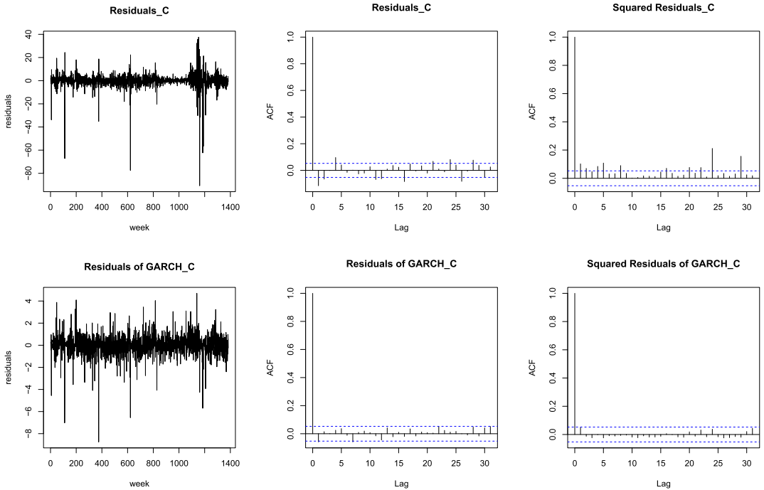
FIG. 3. Time series and autocorrelation plots for Citigroup. The top plots are for the least-squares residuals \{\epsilon_t^{(j)}\} from the model (6.3), and bottom plots are for the corresponding GARCH residual \{\eta_t^{(j)}\} from the model (6.2). The middle plots are for their nominal levels, and right plots are for their squares.
