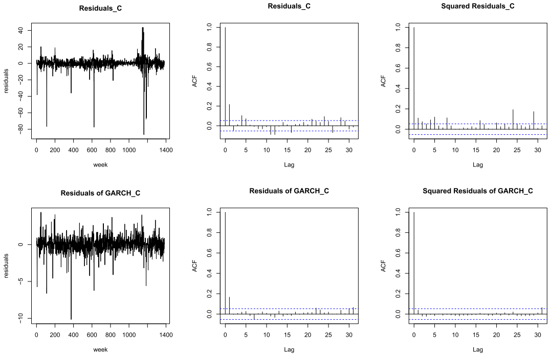
FIG. 2. Time series and autocorrelation plots for Citigroup. The top plots are for the least-squares residuals \{\epsilon_t^{(j)}\} from the model (6.1), and bottom plots are for the corresponding GARCH residual \{\eta_t^{(j)}\} from the model (6.2). The middle plots are for their nominal levels, and right plots are for their squares.
