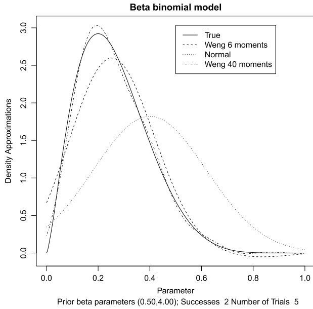
FIG. 1. Density approximation of Weng [50].
