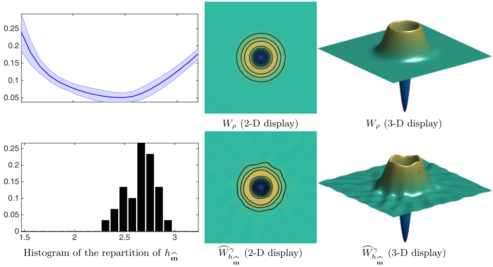
FIG. 1. Single photon cat state estimation, with \eta = 0.9 , n = 100 \times 10^3 . Left, top: display of \|\widehat{W}_h^\gamma - W_\rho\|_\infty / \|W_\rho\|_\infty as a function of 1/h . The central curve is the mean of this quantity, while the shaded area displays the \pm 2 \times standard deviation of this quantity. Left, bottom: histogram of the empirical repartition of \widehat{\mathbf{m}} computed by the Lepski procedure (30). Center: display as a 2-D image using level sets of W_\rho (top) and \widehat{W}_{\widehat{\mathbf{m}}}^\gamma (bottom). Right: same, but displayed as an elevation surface.
