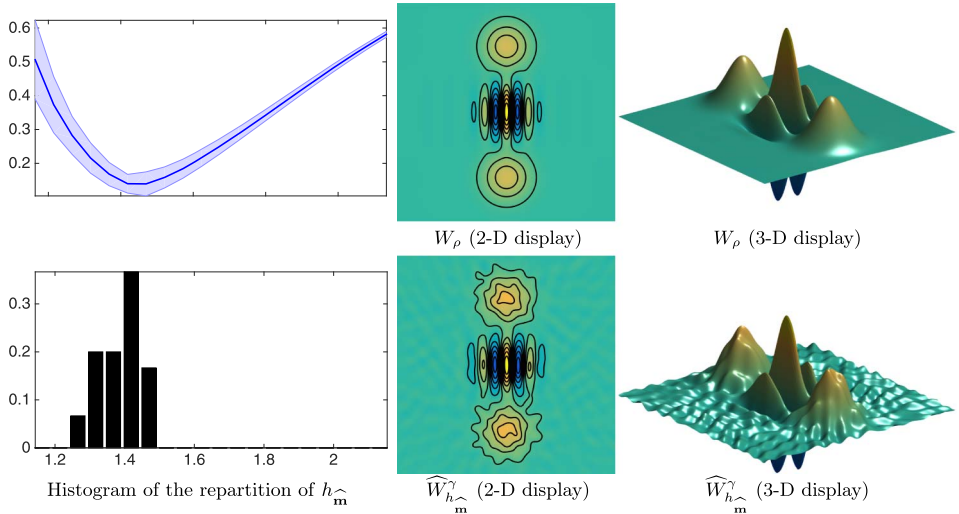
FIG. 2. Schrödinger's cat state estimation, with \eta = 0.9 , n = 500 \times 10^3 . We refer to Figure 1 for the description of the plots.
