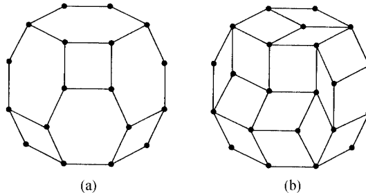
FIG. 9. Two zonotopal tilings of a 12-gon.
