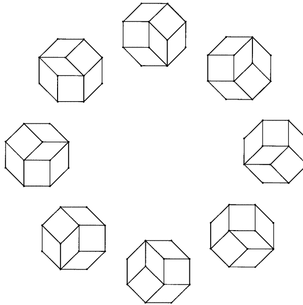
FIG. 10. An octagon of tilings of an octagon.
