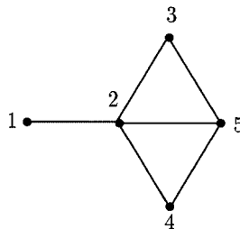
FIG. 8. A threshold graph.
