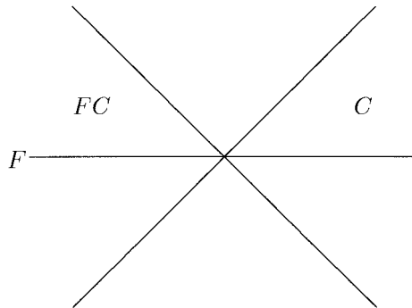
FIG. 2. The projection of C on F .
