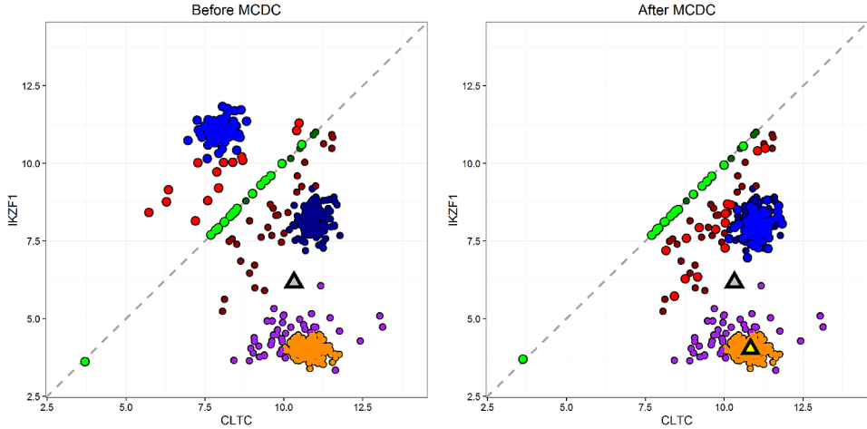
FIG. 13. Example 3 showing the results of applying MCDC to L1000 control data. MCDC chooses 5 clusters by BIC. On the left is the data before correction, and on the right is the same data after correction. Triangles indicate inferred mean; gray is the mean of all the data while yellow is the mean of the largest cluster found by MCDC.
