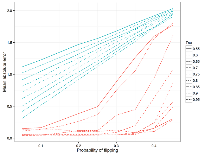
FIG. 7. Mean absolute error in inferred mean comparison for simulation 2 when varying \tau , the probability that a point comes from the primary cluster. The blue line is using unaltered data, while the red line is using the mean of the largest cluster found by MCDC.
