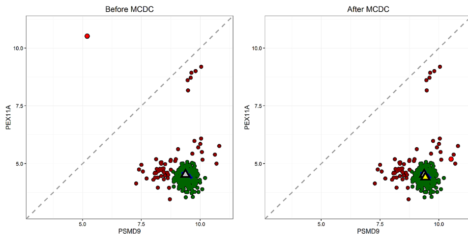
FIG. 11. Example 1 showing the results of applying MCDC to L1000 control data. MCDC chooses 3 clusters by BIC. On the left are the data before correction, and on the right are the same data after correction. Triangles indicate inferred mean; gray is the mean of all the data while yellow is the mean of the largest cluster found by MCDC.
