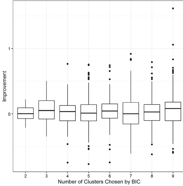
FIG. 15. Boxplots showing the improvement in gene expression estimation for each gene versus the Affymetrix baseline, by the number of clusters chosen. Improvement is calculated as the absolute residual from regression using the original data minus the absolute residual from regression using the MCDC estimates. Positive values indicate improvement from using MCDC.
