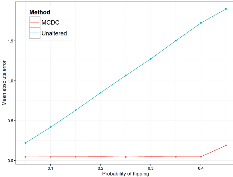
FIG. 5. Simulation 1: Mean Absolute Error in Inferred Mean. The blue line is based on using unaltered data, while the red line is based on using the mean of the largest cluster found by MCDC.
