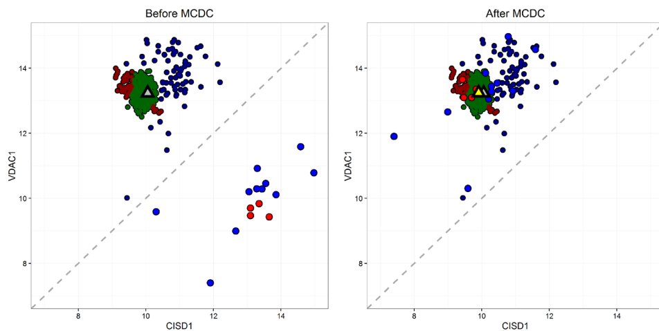
FIG. 12. Example 2 showing the results of applying MCDC to L1000 control data. MCDC chooses 3 clusters by BIC. On the left is the data before correction, and on the right is the same data after correction. Triangles indicate inferred mean—gray is the mean of all the data while yellow is the mean of the largest cluster found by MCDC.
