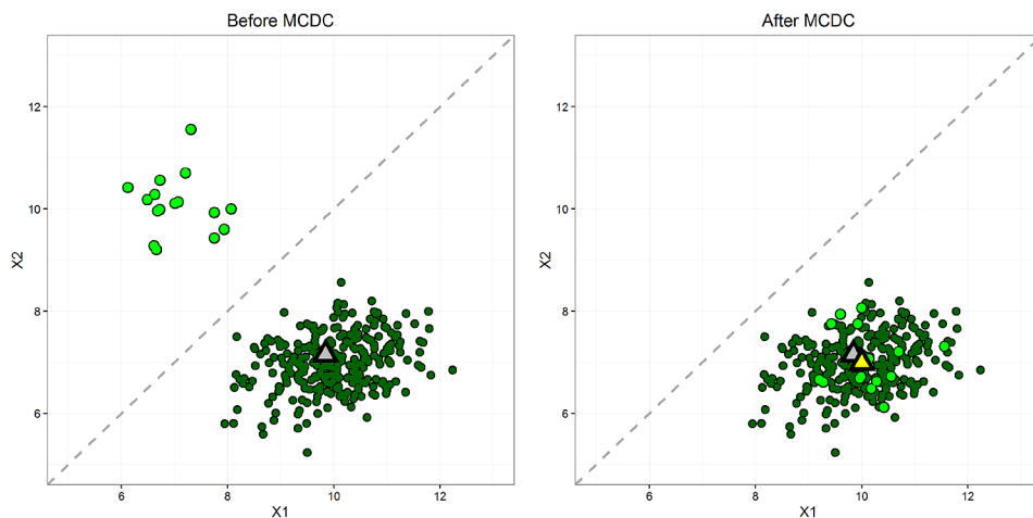
FIG. 4. One Dataset from Simulation 1: One Cluster with Flipping. The fraction of data flipped, 1 - \pi , is chosen to be 0.05. Left panel: Original data with flipped data points. Right panel: Data after correction by MCDC. MCDC identified and corrected all the flipped points. The gray triangle is the mean of all the data, and the yellow triangle is the mean of the data after correction by MCDC.
