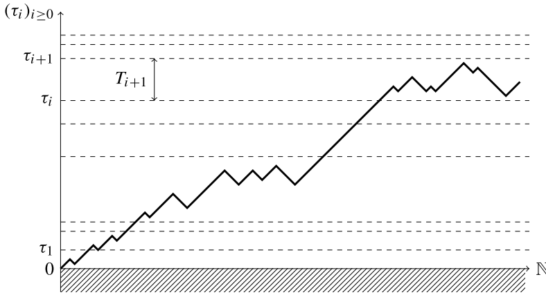
FIG. 1. Example of a polymer among repulsive interfaces. The dashed lines correspond to the interfaces, the thick one to the polymer and the shaded area to the hard wall.
