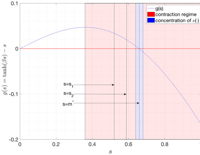
FIG. 1. g(s) for \beta = 1.2 .
