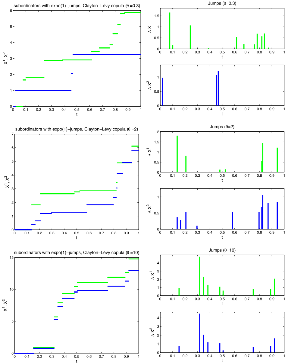
FIG. 1. Simulations of CPPs (X^1, X^2) with expo(1)-distributed jump sizes and dependence modeled by a Clayton-Lévy copula for \theta = 0.3 , \theta = 2 and \theta = 10 ; left-hand side: sample paths of CPP, right-hand side: CPP as marked point process. When \theta increases, then the number of single jumps \Delta P^1 , \Delta P^2 , cf. (3.4), decreases and the number of common jumps \Delta P^3 increases. Further, for increasing \theta , the dependence between jump sizes of X^1 and X^2 increases.
