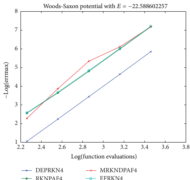
FIGURE 7: Efficiency for the Schrödinger equation using E = -22.588602257 .
