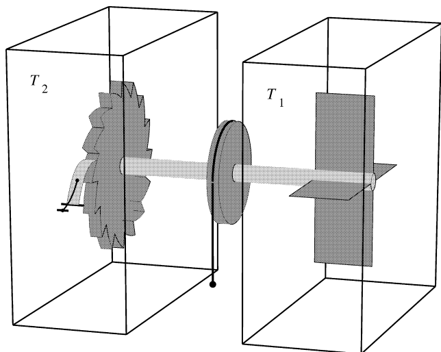
FIG. 1. The ratchet and pawl machine. There are two boxes with a vane in one and a wheel that can only turn one way, a ratchet and pawl, in the other. Each box is in a thermal bath of gas molecules at equilibrium. The two boxes are connected mechanically by a thermally insulated axle. The whole device is considered to be reduced to microscopic size so gas molecules can randomly bombard the vane to produce motion.
