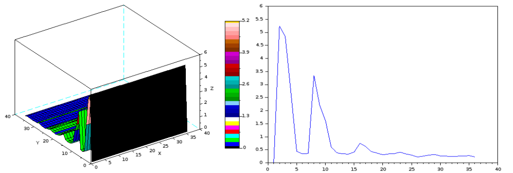
FIGURE 2. DISTRIBUTION OF THE FIRST TERM CORRECTOR Z^1(t, \frac{t}{\epsilon}, \cdot, \cdot) 3D IN THE LEFT AND 2D IN THE RIGHT FOR t = \frac{1}{3} , \epsilon = 0.01 . Distribution of the first term corrector Z^1(t, \frac{t}{\epsilon}, \cdot, \cdot) 3D in the left and 2D in the right for t = \frac{1}{3} , \epsilon = 0.01 .
