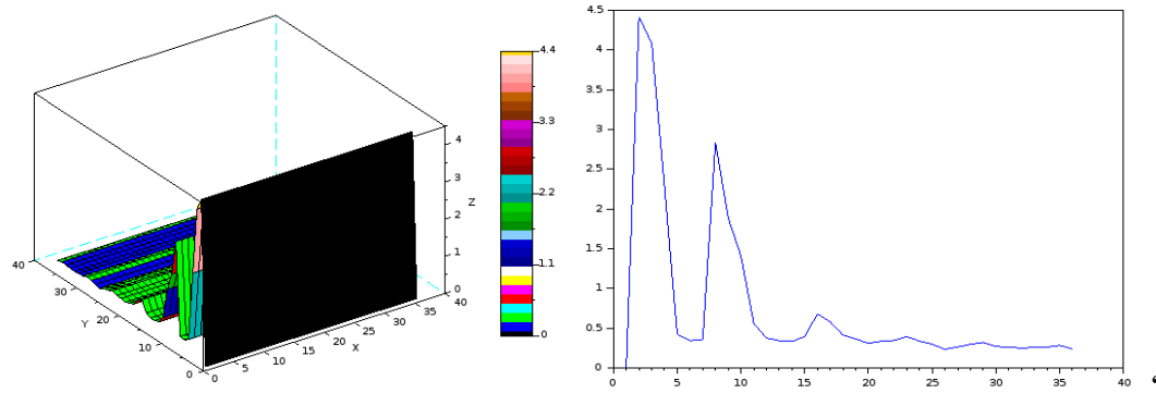
FIGURE 3. DISTRIBUTION OF THE FIRST TERM CORRECTOR Z^1(t, \frac{t}{\epsilon}, \cdot, \cdot) 3D IN THE LEFT AND 2D IN THE RIGHT FOR t = \frac{1}{4} , \epsilon = 0.01 .. Distribution of the first term corrector Z^1(t, \frac{t}{\epsilon}, \cdot, \cdot) 3D in the left and 2D in the right for t = \frac{1}{4} , \epsilon = 0.01 .
