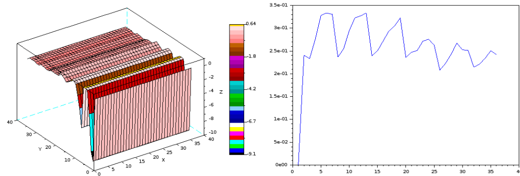
FIGURE 8. APPROXIMATION OF THE REFERENCE SOLUTION z^\epsilon , FOR \epsilon = 0.01 AT t = \frac{1}{4} , 3D IN THE LEFT AND 2D IN THE RIGHT, Z^0(t, \frac{t}{\epsilon}, \cdot, \cdot) + \epsilon Z^1(t, \frac{t}{\epsilon}, \cdot, \cdot) . Approximation of the reference solution z^\epsilon , for \epsilon = 0.01 at t = \frac{1}{4} , 3D in the left and 2D in the right, Z^0(t, \frac{t}{\epsilon}, \cdot, \cdot) + \epsilon Z^1(t, \frac{t}{\epsilon}, \cdot, \cdot) .
