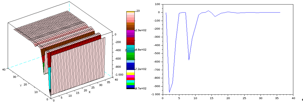
FIGURE 4. DISTRIBUTION OF THE FIRST TERM CORRECTOR Z^1(t, \frac{t}{\epsilon}, \cdot, \cdot) 3D IN THE LEFT AND 2D IN THE RIGHT FOR t = \frac{1}{8} , \epsilon = 0.01 .. Distribution of the first term corrector Z^1(t, \frac{t}{\epsilon}, \cdot, \cdot) 3D in the left and 2D in the right for t = \frac{1}{8} , \epsilon = 0.01 .
