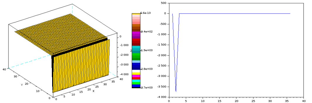
FIGURE 1. DISTRIBUTION OF THE FIRST TERM CORRECTOR Z^1(t, \frac{t}{\epsilon}, \cdot, \cdot) 3D IN THE LEFT AND 2D IN THE RIGHT FOR t = 1 , \epsilon = 0.01 . Distribution of the first term corrector Z^1(t, \frac{t}{\epsilon}, \cdot, \cdot) 3D in the left and 2D in the right for t = 1 , \epsilon = 0.01 .
