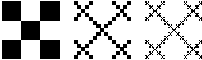
Figure 2: The sets F_1^\xi, F_2^\xi, F_3^\xi when N = 2, L_1 = 1, L_2 = 2, \xi = (1, 2, 1, \dots) .
