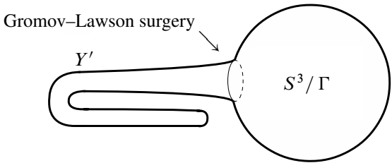
Figure 2: Part of a thin hook, Y' , is glued to S^3 / \Gamma via the Gromov–Lawson procedure.
